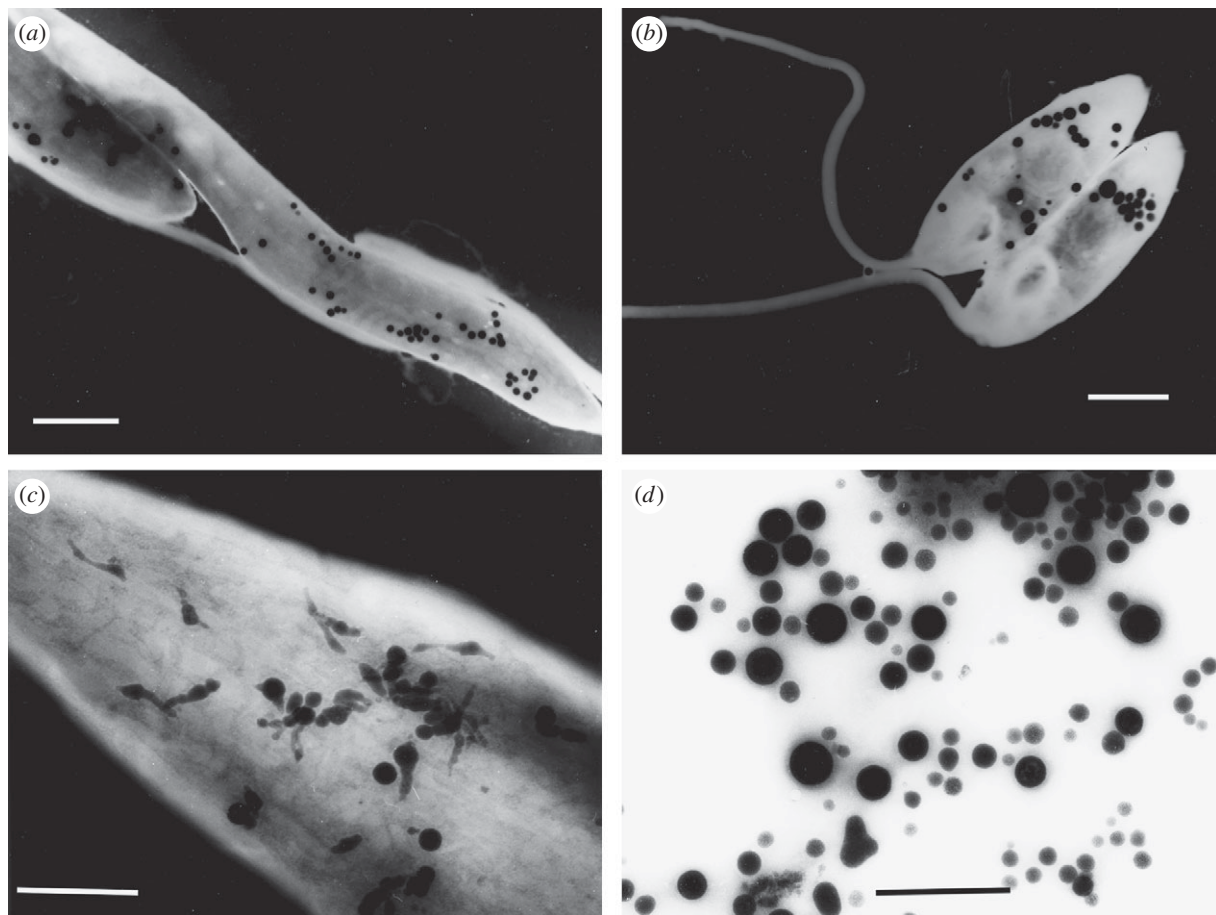
Figure 3. Morphology of trypanosomatid acidocalcisomes. Electron spectroscopic imaging (contrast tuning) of whole cells (a–c) or fractions (d) adhered to formvar-coated grids showing the shape, size and distribution of acidocalcisomes (black spots) in different species. (a) Blastochritidia culicis ; scale bar, 2 \mu\text{m} . (b) Herpetomonas anglusteri ; scale bar, 3 \mu\text{m} . (c) Phytomonas serpens ; scale bar, 0.5 \mu\text{m} . (d) Isolated acidocalcisomes from Trypanosoma cruzi ; scale bar, 0.5 \mu\text{m} . Note the polymorphic nature of acidocalcisomes in (c). b,c are adapted from Miranda et al. (2004, Copyright Elsevier).
