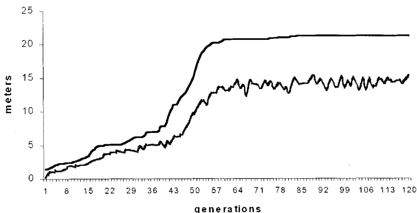
Fig. 6. Fitness graph of representative stable controller evolution. Top fitness (black) and average fitness (grey) are shown.
