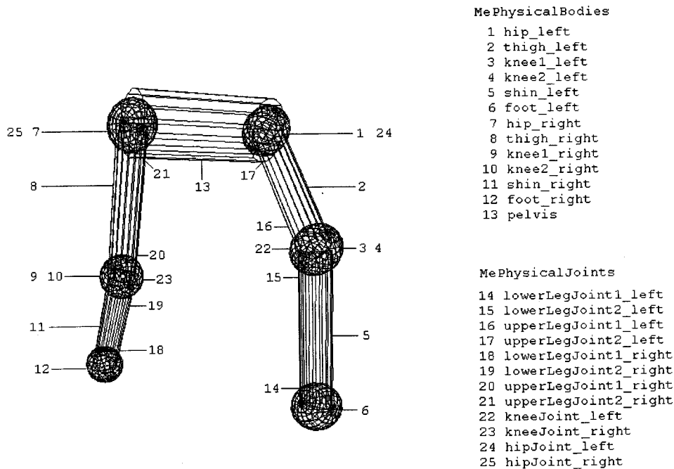
Fig. 1. MathEngine implementation of the biped. Note that although two bodies are used to implement the knee, only one body is necessary.
