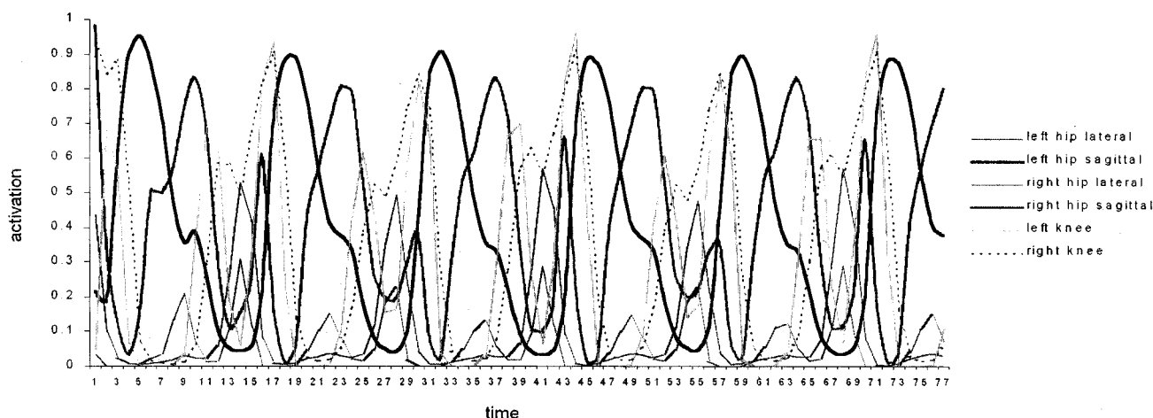
Fig. 7. Motor neuron activation levels of top individual of generation 120 (see Fig. 6).
