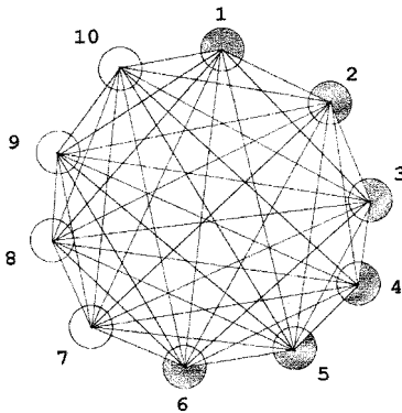
Fig. 2. Recurrent neural network used to control bipedal walking. Shaded nodes are motor neurons. Connections are bidirectional and asymmetric.
