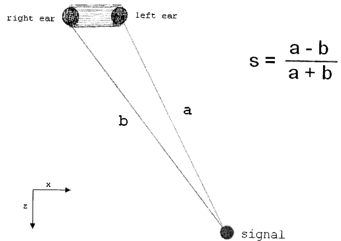
Fig. 9. Preprocessing of two signal values ( a and b ) resulting in final signal value s . Difference is divided by the sum of the two signal strengths to give a stronger directional signal close to the sound source. This also causes the signal to vanish with the biped facing the sound source.
