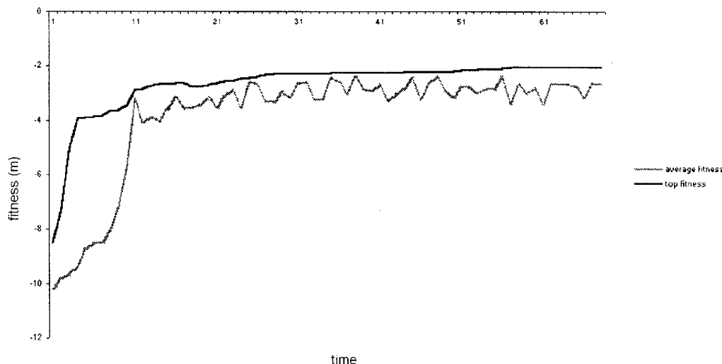
Fig. 11. Fitness graph of bipedal walking with sensory integration. Population was seeded with individuals from the run depicted in Fig. 7.
