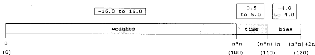
Fig. 4. Encoding scheme. Chromosome index is shown in general form ( n is the number of nodes) and for special case of n = 10 (in brackets). Parameters are encoded as real values. Ranges in the boxes represent upper and lower bounds of the respective parameter types.
