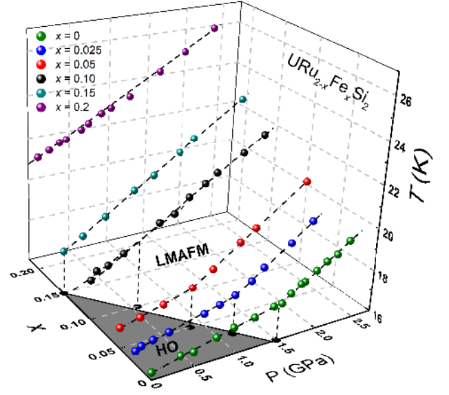
FIG. 7. (Color online) Plot of the T_0 vs. P phase boundaries for various values of x for \text{URu}_{2-x}\text{Fe}_x\text{Si}_2 ( x = 0, 0.025, 0.05, 0.10, 0.15, \text{ and } 0.20 ). The vertical dashed lines drop down to the x - P plane at the respective critical pressures P_c and help determine the boundary between the HO and LMAFM phases in the x - P plane. The HO/LMAFM phase boundary is represented by the solid black line in the x - P plane which is a linear fit of the black circles. At the critical concentration of x_c^* = 0.15 and above, the compounds have already entered the LMAFM phase at ambient pressure. (The green data points shown for x = 0 are not part of this study and were taken from an earlier study of \text{URu}_{2-x}\text{Fe}_x\text{Si}_2 under pressure by Jeffries et al. in Ref. 19.)
