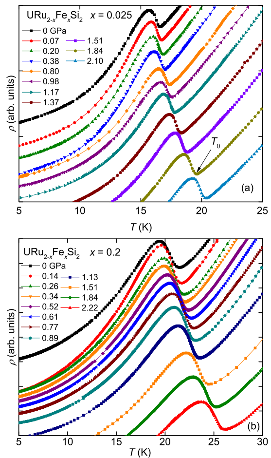
FIG. 3. (Color online) Temperature dependence of electrical resistivity \rho(T) near the HO/LMAFM transition temperature T_0 at various pressures for URu_{2-x}Fe_xSi_2 (a) x=0.025 and (b) x=0.2 . The \rho(T) curves have been shifted vertically for clarity in illustrating the evolution of the resistivity feature near T_0 . (Electrical resistivity curves for the other Fe concentrations, x = 0.05, 0.10, 0.15 , are not shown but exhibit similar behavior). The transition temperature T_0 is defined as the temperature at which there is a minimum in \rho(T) as indicated by the black arrow in the upper panel.
