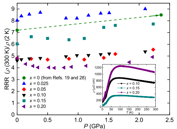
FIG. 2. (Color online) A plot of the residual resistivity ratio ( \text{RRR} = \rho(300 \text{ K})/\rho(2 \text{ K}) ) as a function of pressure, P , for single crystal samples of \text{URu}_{2-x}\text{Fe}_x\text{Si}_2 at x = 0, 0.025, 0.05, 0.10, 0.15, and 0.20 . The two green data points for the x = 0 sample at P = 0 and 2.4 GPa connected by the dashed green arrow are taken from Refs. 19 and 28. Inset: A plot of the “unshifted” \rho vs. T curves at ambient pressure for the \text{URu}_{2-x}\text{Fe}_x\text{Si}_2 ( x = 0.10, 0.15, and 0.20 ) compounds, which displays the drop in the nominal electrical resistivity for the x = 0.15 compound relative to the neighboring concentrations of x = 0.10 and 0.20 .
