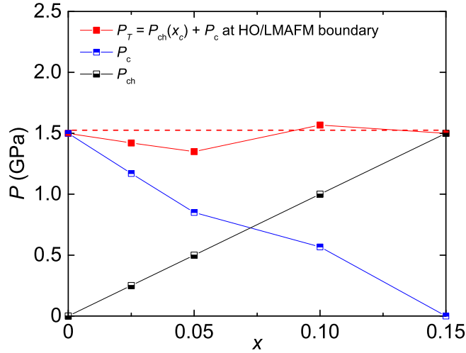
FIG. 8. (Color online) A plot of the chemical pressure P_{ch} (black symbols), critical applied pressure P_c (blue symbols), and the total pressure P_T (red symbols) = P_{ch}(x_c) + P_c . The additive behavior of P_{ch} and P_c such that P_{ch}(x_c) + P_c \approx 1.5 GPa is consistent with earlier reports on the “kink” in the T_0(P) phase diagram at P = 1.5 GPa for the parent compound \text{URu}_2\text{Si}_2 ( x = 0 ). 19
