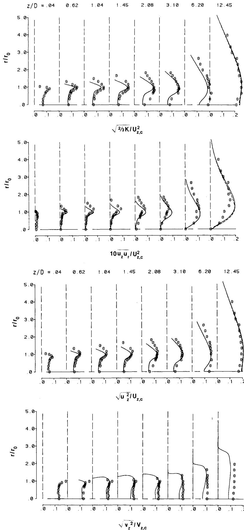
Fig. 8 Radial profiles of normalized gas turbulence kinetic energy, shear stress, and axial turbulence intensity, and particle axial turbulence intensity at loading ratio, LR = 0.2; --- stochastic treatment, — deterministic treatment.
