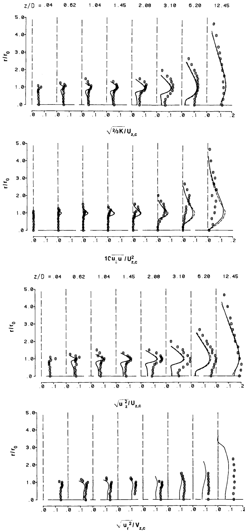
Fig. 11 Radial profiles of normalized gas turbulence kinetic energy, shear stress, and axial turbulence intensity, and particle axial turbulence intensity at loading ratio, LR = 1.0; --- stochastic treatment, — deterministic treatment.
