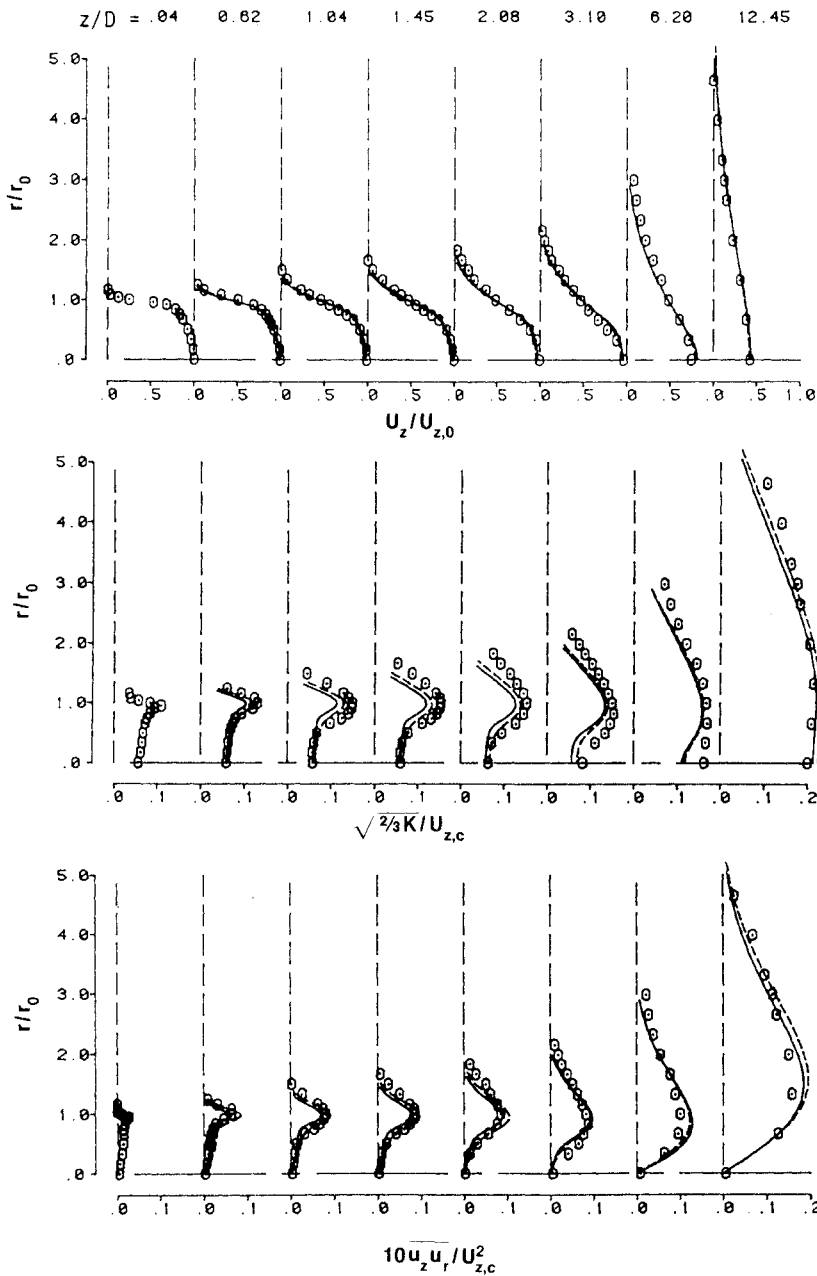
Fig. 5 Radial profiles of normalized mean axial velocity, turbulence kinetic energy, and shear stress for the single-phase jet; influence of initial \epsilon ; - - - \epsilon_{inlet} = \epsilon_0 , — \epsilon_{inlet} = 0.5 \epsilon_0 .
