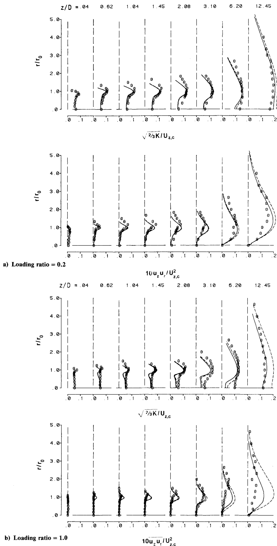
Fig. 13 Effect of single-phase and two-phase turbulence models on gas phase turbulence kinetic energy and shear stress for the two loading ratios, LR = 0.2 and 1.0; - - - two-phase model, — single-phase model.
