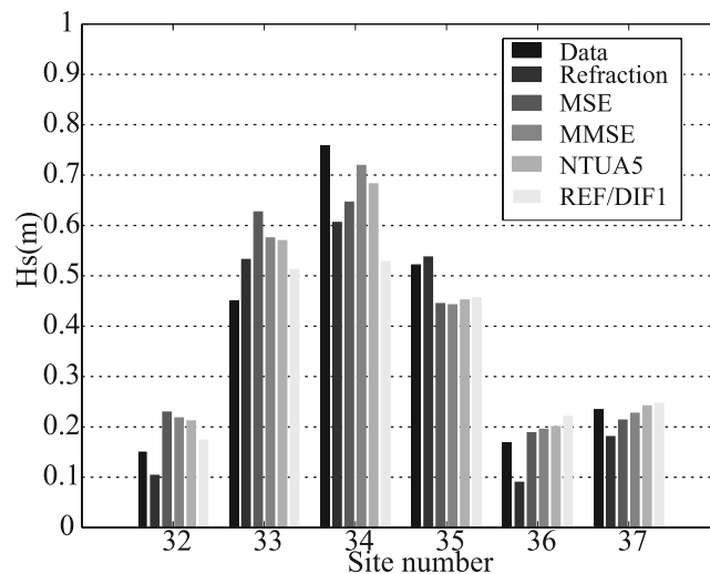
Figure 15. Comparison of predicted and observed significant wave height ( 12 \text{ s} < T < 22 \text{ s} ) for the 12 December 2003 swell event. Instrument locations are shown in Figure 9.
