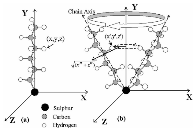
FIG. 4. The structure of the monolayer on the surface of a metal particle. The S atom is on the surface of the particle. (a) Molecular axis of the alkyl chain is oriented along the Y axis and is rotated around it (model M1). (b) Molecular axis is rotated through an angle \theta about Z axis (model M2). Molecular axis is shown to undergo a rotation in a cone around the Y axis. Origin is located at the sulfur atom and is assumed to be fixed. \sqrt{(x'^2 + z'^2)} = r , is the radius of gyration.
