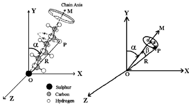
FIG. 5. A hydrogen atom at P is moving with respect to the chain axis (OM). Chain axis, OM fluctuates around the Y axis (model M3).
