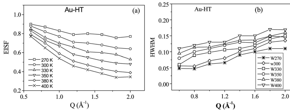
FIG. 3. (a) The extracted EISF and (b) width of the quasielastic part as obtained from the fit with experimental data for Au-HT at different temperatures. The continuous evolution of the alkyl-chain dynamics is evident. Lines are guides to the eye.
