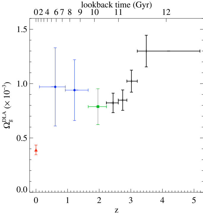
Fig. 17. Cosmological mass density of neutral gas in DLAs, \Omega_g^{\text{DLA}} , as a function of redshift. The red triangle at z = 0 is the value from 21-cm maps by Zwaan et al. (2005b). The blue filled circles at z \sim 1 are the measurements of \Omega_g^{\text{DLA}} from Rao et al. (2006). The green square at z \sim 2 is derived from the sample of Péroux et al. (2003). Measurements at z > 2.2 are from the present work based on SDSS DR7.
