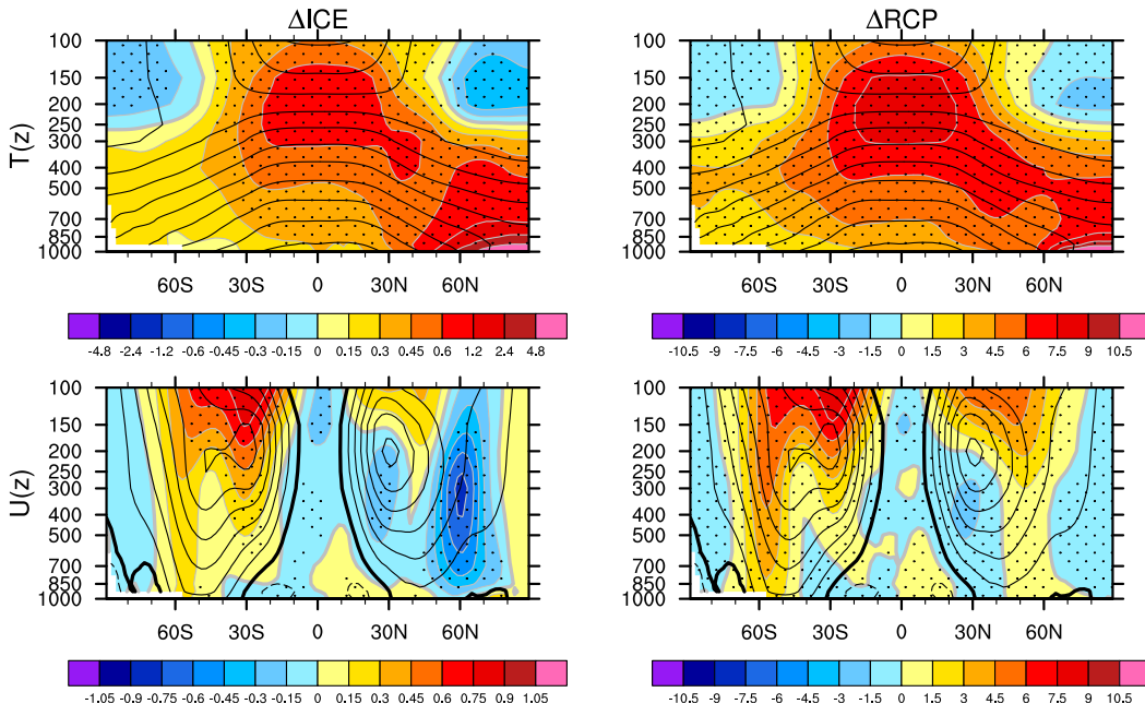
FIG. 13. (top) Annual zonal-mean temperature ( ^{\circ}\text{C} ) response in (left) \Delta\text{ICE} and (right) \Delta\text{RCP} averaged over 2051–90, overlaid by the climatology (contours). The contour interval is 10^{\circ}\text{C} . (bottom) As in (top), but for zonal-mean zonal wind ( \text{m s}^{-1} ) response. Contour interval is 5 \text{ m s}^{-1} . Stippling denotes the 95% statistical significance based on a two-sided Student's t test.
