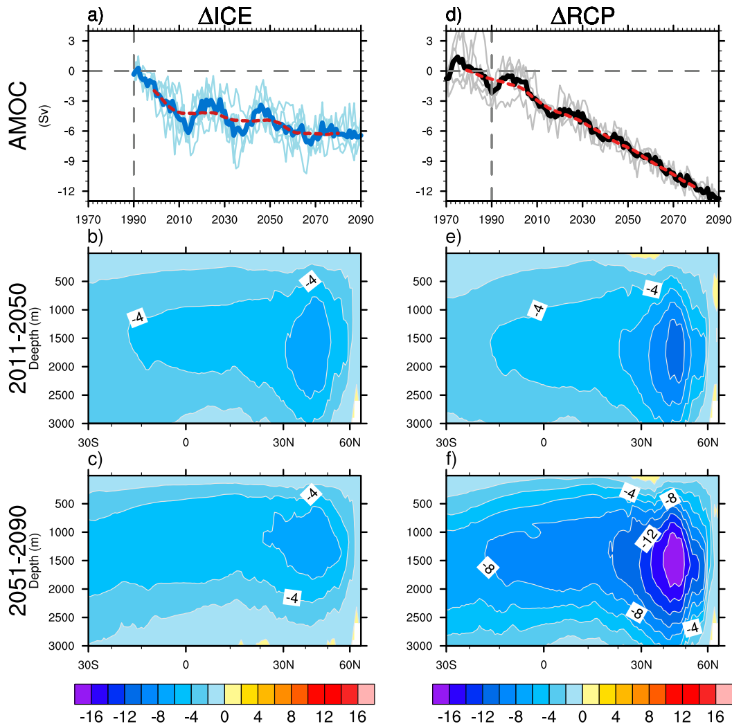
FIG. 4. (a),(d) Time series of AMOC response (in Sv) in \Delta ICE and \Delta RCP, respectively. Thin blue curves denote the individual members and thick blue curve indicate ensemble mean. Dashed red curve indicates the smoothed blue curve using 20-yr running mean. (b),(e) Latitude–depth cross section of the AMOC streamfunction averaged over 2011–50 in \Delta ICE and \Delta RCP, respectively. (c),(f) As in (b),(e), but averaged over 2051–90. Contour interval is 2 Sv.
