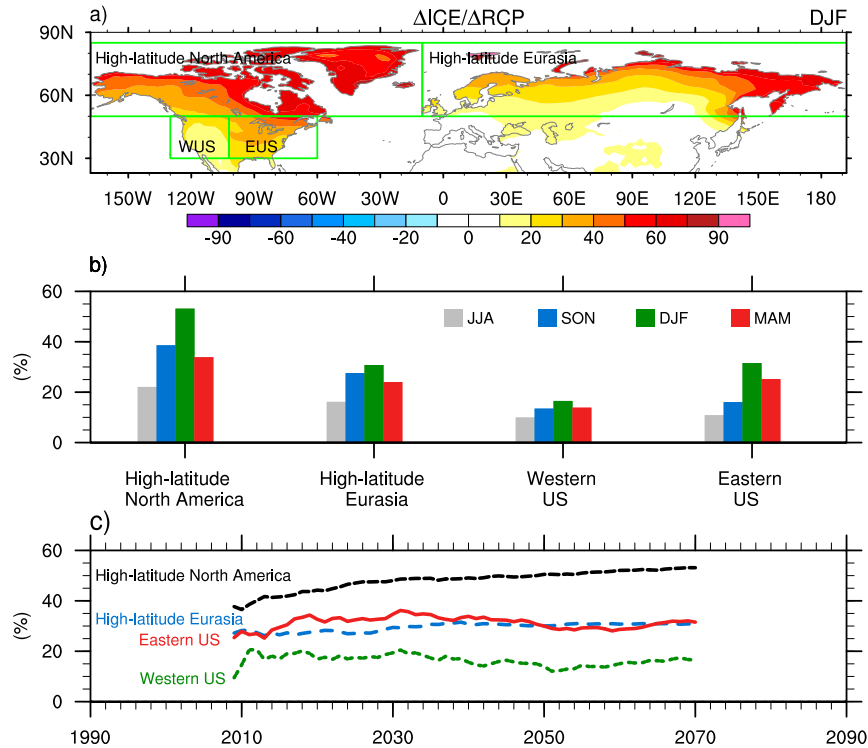
FIG. 10. (a) Fraction (%) of \Delta\text{ICE}/\Delta\text{RCP} for winter near-surface air temperature response in 2051–90. Green boxes denote various high-latitude and midlatitude continents, including high-latitude North America, high-latitude Eurasia, western United States (WUS), and eastern United States (EUS). (b) As in (a), but averaged over four individual continents in JJA (gray bars), SON (light blue bars), DJF (green bars), and MAM (red bars). (c) As in (b), but for the time evolution of winter temperature response fractions. To remove the internal variability, 40-yr running mean is first performed before calculating the fraction.
