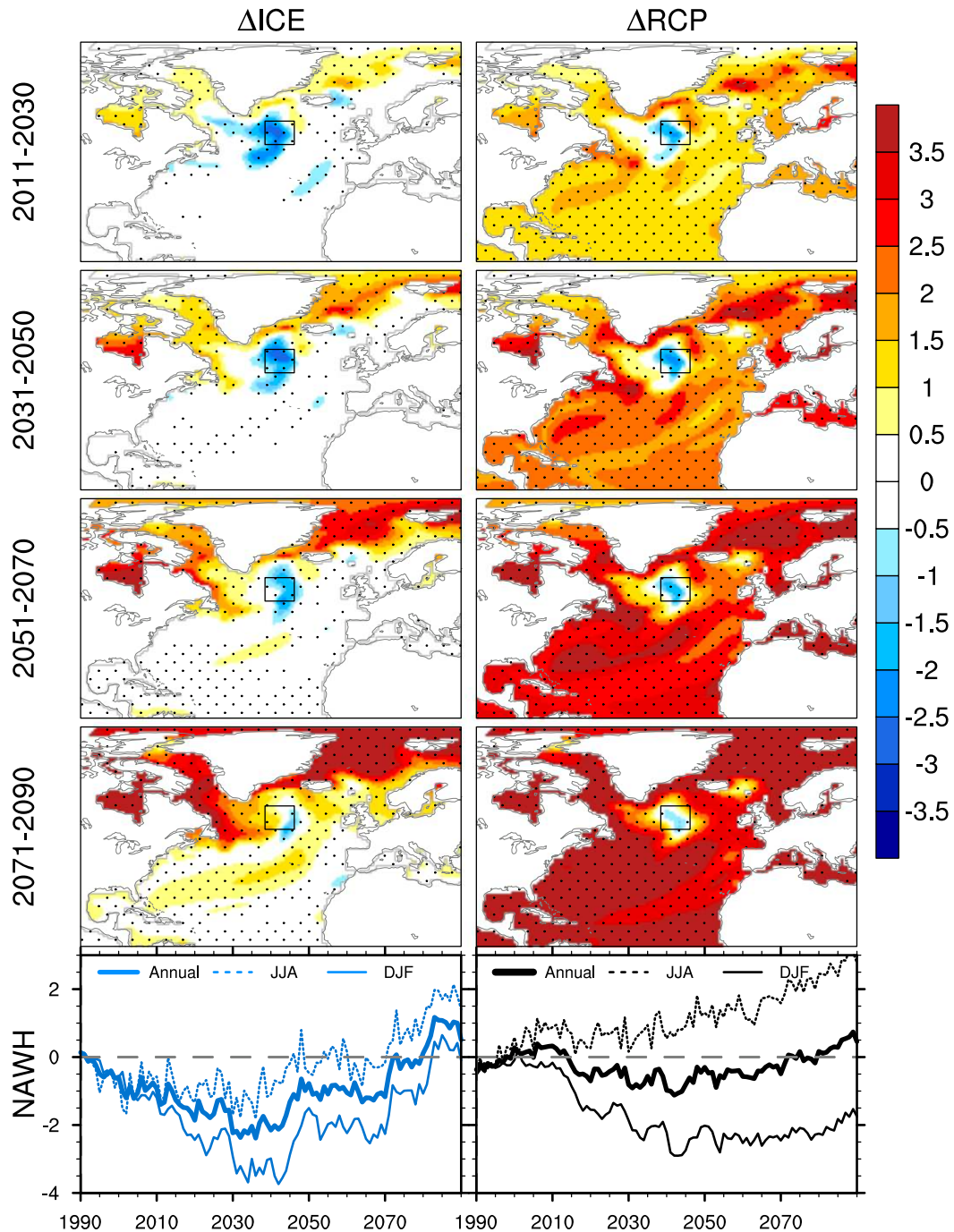
FIG. 5. (top four rows) Annual North Atlantic SST responses in (left) \Delta ICE and (right) \Delta RCP averaged over 2011–30, 2031–50, 2051–70, and 2071–90. Black boxes indicate the North Atlantic warming hole (NAWH; 50°–60°N, 27°–37°W). (bottom) Time series of the NAWH annual (thick curve) and JJA and DJF (thin curve) SST responses in (left) \Delta ICE and (right) \Delta RCP. Stippling denotes the 95% statistical significance based on two-sided Student's t test.
