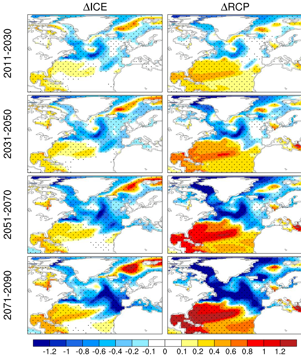
FIG. 6. As in Fig. 5 (top four rows), but for the annual North Atlantic sea surface salinity (SSS; psu) responses in (left) \Delta ICE and (right) \Delta RCP averaged over 2011–30, 2031–50, 2051–70, and 2071–90. Stippling denotes the 95% statistical significance based on a two-sided Student's t test.
