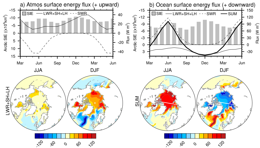
FIG. 2. (a) (top) Monthly change of SIE between 1971–90 and 2051–90 (gray bars; 10^6 \text{ km}^2 ), and Arctic atmospheric surface energy flux ( \text{W m}^{-2} ; positive upward) response in \Delta \text{ICE} (obtained by differencing the RCP and RCP_ICE1990 and averaged over the climatological March SIE region) during 2051–90. Atmospheric surface energy flux includes longwave radiative flux (LWR), sensible heat (SH), and latent heat (LH) flux. Shortwave radiative flux (SWR) is displayed separately. (bottom) Atmospheric surface energy flux response in (left) JJA and (right) DJF. (b) As in (a) but for the ocean surface energy flux response (positive downward). Ocean surface energy flux includes SWR, LWR, SH, and LH. Contour interval is 20 \text{ W m}^{-2} . Note that (a) is obtained from atmosphere model output and (b) is obtained from ocean model output. White lines in the bottom panel of (b) are due to polar projections on tripolar grids.
