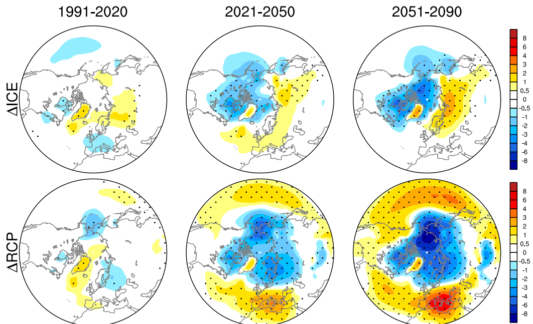
FIG. 8. (a) Winter (DJF) 500-hPa geopotential height (m) responses in \Delta ICE and \Delta RCP for 1991–2020, 2021–50, and 2051–90. (b) As in (a), but for the sea level pressure (hPa) responses. Stippling denotes the 95% statistical significance based on a two-sided Student's t test.
