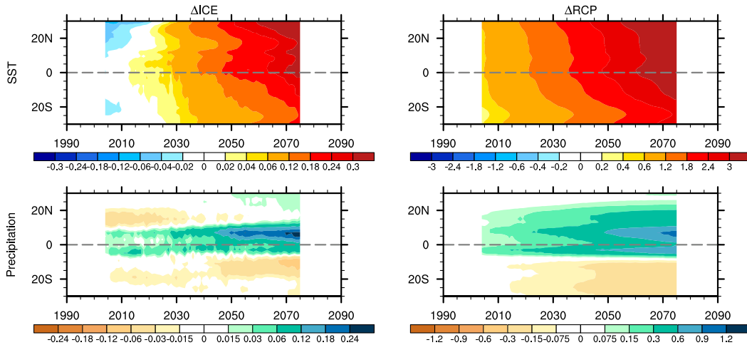
FIG. 12. (top) Annual tropical zonal-mean SST ( ^{\circ}\text{C} ) response as a function of time and latitude in (left) \Delta\text{ICE} and (right) \Delta\text{RCP} . (bottom) As in (top), but for annual tropical zonal-mean precipitation ( \text{mm day}^{-1} ) response. To remove internal variability, SST and precipitation responses have been smoothed by 30-yr running mean. Note that the color scales are different between \Delta\text{ICE} and \Delta\text{RCP} .
