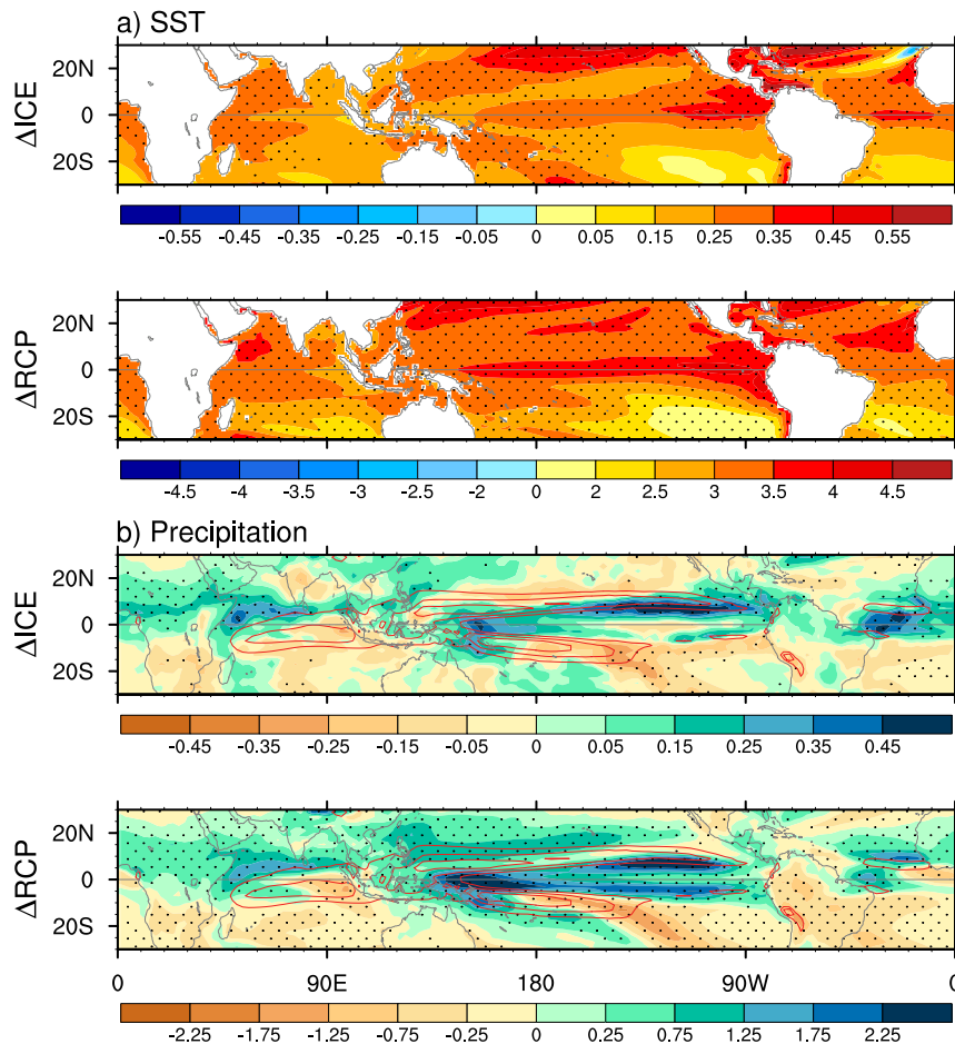
FIG. 11. (a): Annual tropical SST ( ^{\circ}\text{C} ) response in \Delta\text{ICE} and \Delta\text{RCP} averaged over 2051–90. (b) As in (a), but for precipitation ( \text{mm day}^{-1} ) response, overlaid by its climatology. Stippling denotes the 95% statistical significance based on a two-sided Student's t test.
