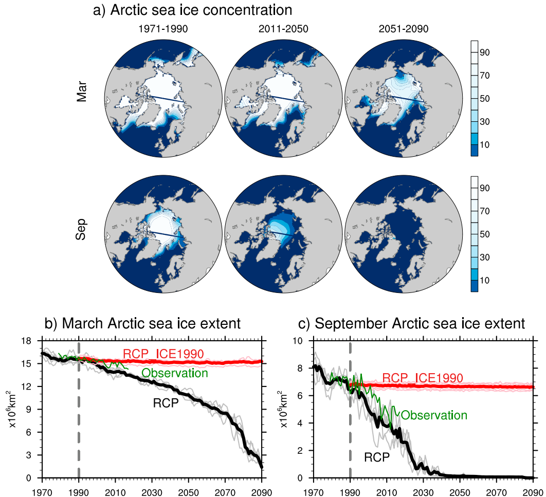
FIG. 1. (a) Arctic sea ice concentration (%) averaged over (left) 1971–90, (middle) 2011–50, and (right) 2051–90 in RCP experiments. (b) March Arctic sea ice extent ( 10^6 \text{ km}^2 ) from CM3 RCP and RCP_ICE1990 experiments. (c) As in (b), but for sea ice extent in September. Thin gray (pink) curves denote the RCP (RCP_ICE1990) individual members and thick curve denotes the ensemble mean. Green curves show the observed values from National Snow and Ice Data Center. Blue lines in (a) are due to polar projections on tripolar grids.
