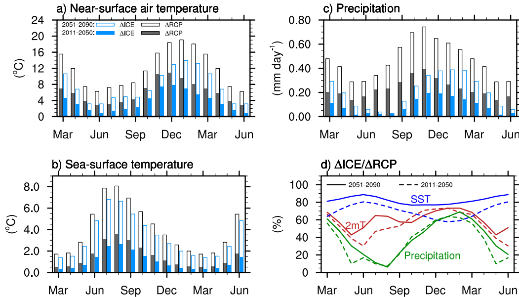
FIG. 3. (a) Monthly change of Arctic near-surface air temperature ( ^{\circ}\text{C} ) responses in \Delta\text{ICE} (blue bars; RCP minus RCP_ICE1990) and \Delta\text{RCP} [black bars; RCP minus RCP(1971–90)] averaged over 2011–50 (filled bars) and 2051–90 (empty bars). (b) As in (a), but for the Arctic sea surface temperature ( ^{\circ}\text{C} ) responses. (c) As in (a), but for the Arctic precipitation ( \text{mm day}^{-1} ) responses. (d) Seasonal cycle of the fraction (%) of \Delta\text{ICE}/\Delta\text{RCP} . In (a)–(c), the Arctic is defined as the region of climatological Arctic sea ice extent in March.
