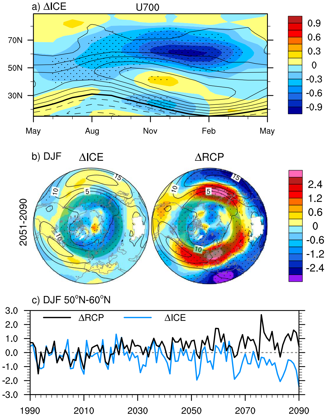
FIG. 7. (a) Monthly change of 700-hPa zonal-mean zonal wind response in \Delta\text{ICE} averaged over 2051–90. Contours denote the climatology with the interval of 2 \text{ m s}^{-1} and zero wind line thickened. (b) Winter (DJF) 700-hPa zonal wind responses in (left) \Delta\text{ICE} and (right) \Delta\text{RCP} . Contours denote the climatology with the interval of 5 \text{ m s}^{-1} . Stippling denotes the 95% statistical significance based on a two-sided Student's t test. The shading rings indicate the 50^\circ\text{--}60^\circ\text{N} latitude band. (c) Time evolution of winter 50^\circ\text{--}60^\circ\text{N} averaged 700-hPa zonal-mean zonal wind responses in \Delta\text{ICE} (blue curve) and \Delta\text{RCP} (black curve).
