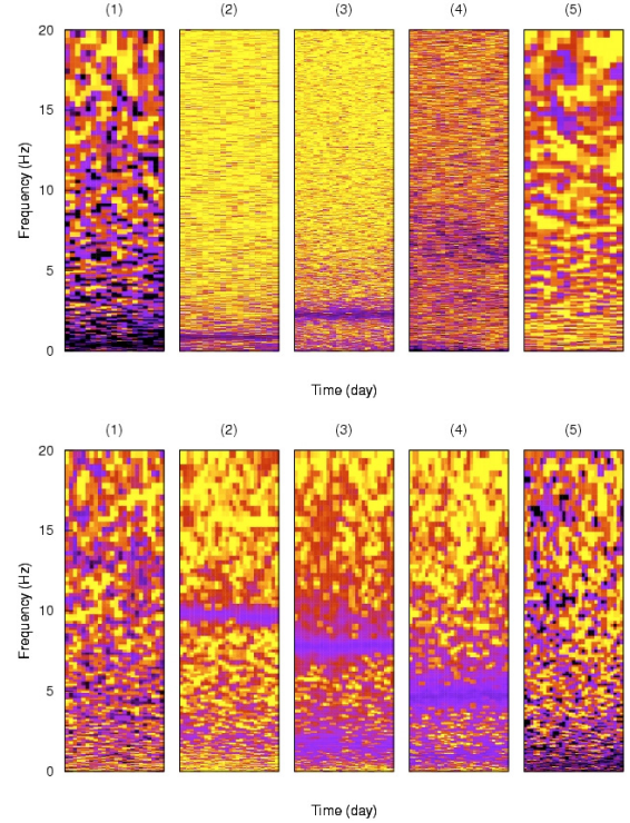
Fig. 2. a) Dynamic power density spectra over five days in the rising phase. (1) Obs. ID = 91404-01-01-01, QPO = 0.382 Hz; (2) Obs. ID = 91702-01-01-03, QPO = 0.886 Hz; (3) Obs. ID = 90704-04-01-00, QPO = 2.3130 Hz; (4) Obs. ID = 91702-01-02-00, QPO = 3.45 and 6.522 Hz with a break frequency at 0.78 Hz and (5) Obs. ID = 91702-01-02-01, QPO = 1 4.54 and 17.78 Hz. b) Dynamic power density spectra over five days in the decline phase. (1) Obs. ID = 91702-01-76-00, QPO = 13.14 Hz; (2) Obs. ID = 9 1702-01-79-01, QPO = 9.77 Hz; (3) Obs. ID = 91702-01-80-00, QPO = 7.823 and 15.2 Hz with a break frequency at 1.32 Hz; (4) Obs. ID = 91702-01-80-01, QPO = 4.732 Hz with a break frequency = 0.86 Hz; (5) Obs. ID = 91702-01-82-00, QPO = 0.423 Hz.
