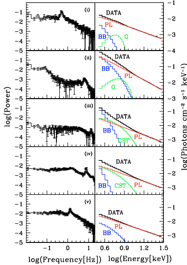
Fig. 3. Power density spectrum ( left panel ) and energy spectral index ( right panel ) of the rising phase (i and ii) and the declining phase (iii–v). The QPO frequencies are (i) 0.513 Hz (0.632); (ii) 3.45 and 6.522 Hz (0.441); (iii) 13.14 Hz (0.848); (iv) 7.823 Hz (1.14) and (v) 1.347 Hz (1.29) respectively. Numbers next to frequencies are the reduced \chi^2 values. The components used for fitting the energy spectra are marked: “DATA” for total fit, “BB” for black body, “G” for Gaussian, “CST” for Comptonization using the Sunyaev-Titarchuk (1980) model with an exponential cutoff, “PL” for a power-law component without a cut-off.
