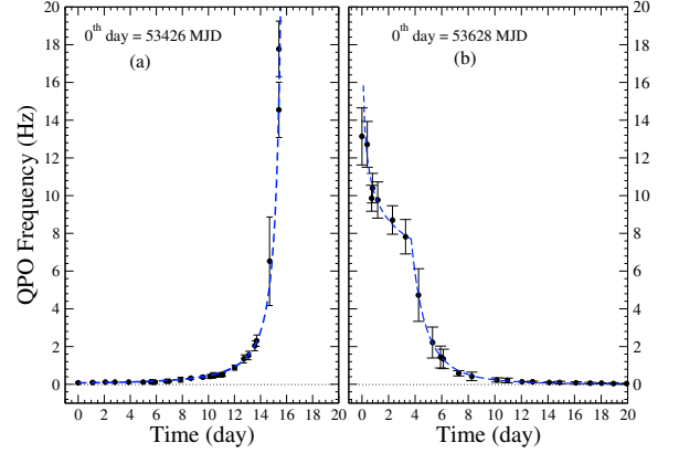
Fig. 1. Variation of QPO frequency with time (in day) a) of the rising phase and b) of the declining phase. Error bars are FWHM of fitted Lorentzian curves in the power density spectrum. The dotted curves are the solutions from oscillating and propagating shocks. While in a) the shock appears to be drifting at a constant speed towards the black hole, in b) the shock initially moves very slowly and then extends at a roughly constant acceleration. According to the fitted solution, the shock wave goes behind the horizon on the 16.14th day, about 15 h after the last observed QPO.
