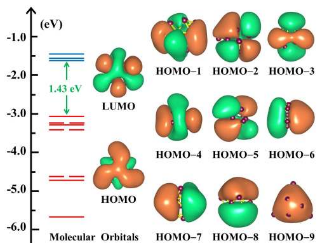
Figure 4. Molecular orbitals and energy levels of neutral \text{Na}_{20} cluster. The HOMO-LUMO energy gap is indicated (in green).
