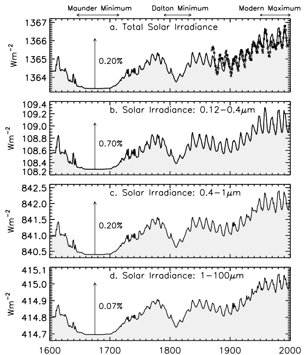
Figure 4. Compared are reconstructions of annual total irradiance in a) with spectral irradiance in broad bands from b) 0.12\text{--}0.4 \mu\text{m} , c) 0.4\text{--}1 \mu\text{m} and d) 1\text{--}100 \mu\text{m} . The summed bands in b), c) and d) equal the total irradiance variations in a). The shading identifies 11-year running means and the arrows show percentage increases from 1675 to the mean of cycle 22 (1986-1996). The symbols in a) are estimates of total irradiance (scaled by 0.999) determined independently by Lockwood and Stamper [1999].
