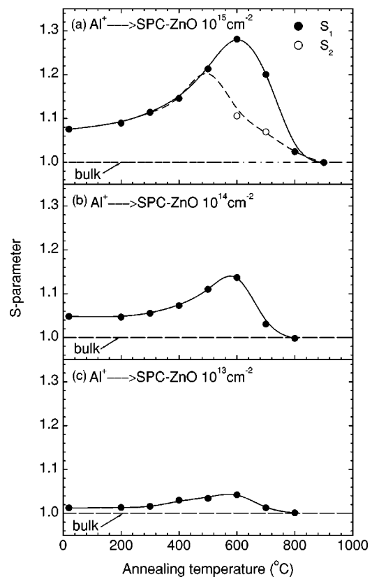
FIG. 8. S parameter in the defect layers as a function of annealing temperature for the Al + -implanted ZnO. For the sample implanted with a dose of 10^{15} Al + /cm 2 , two defect layers appear after annealing at 600–700 °C. S_1 and S_2 are the S parameters in the first and second defect layer, respectively.
