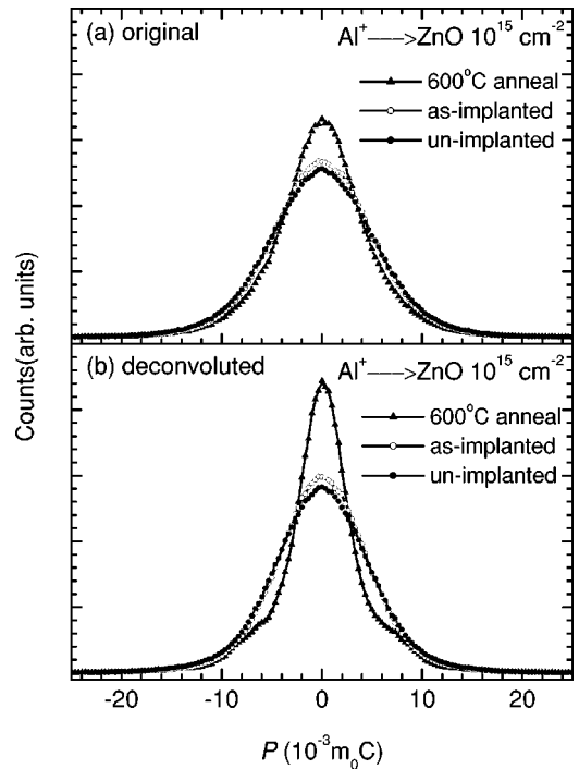
FIG. 10. (a) Original and (b) deconvoluted Doppler broadening spectra for the ZnO before and after \text{Al}^+ implantation ( 10^{15} \text{ Al}^+/\text{cm}^2 ) and 600 °C annealing. The original spectrum is obtained by summing of the spectra at energy of 5–9 keV. The appearance of a narrow component after implantation and annealing indicates formation of p-Ps.
