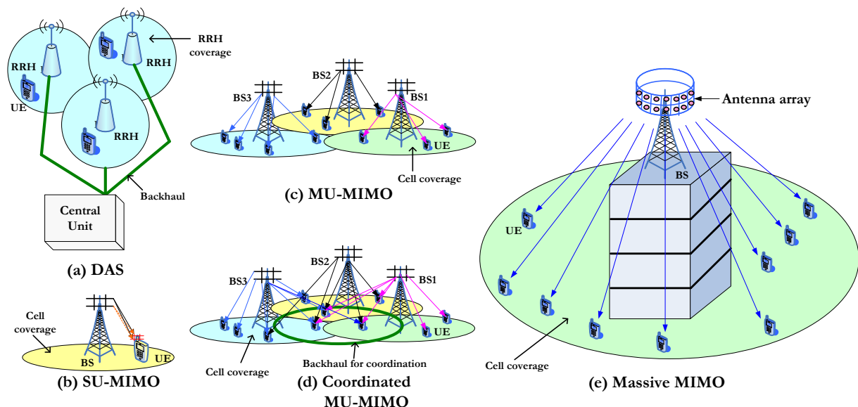
Fig. 5. Multi-antenna configurations.
