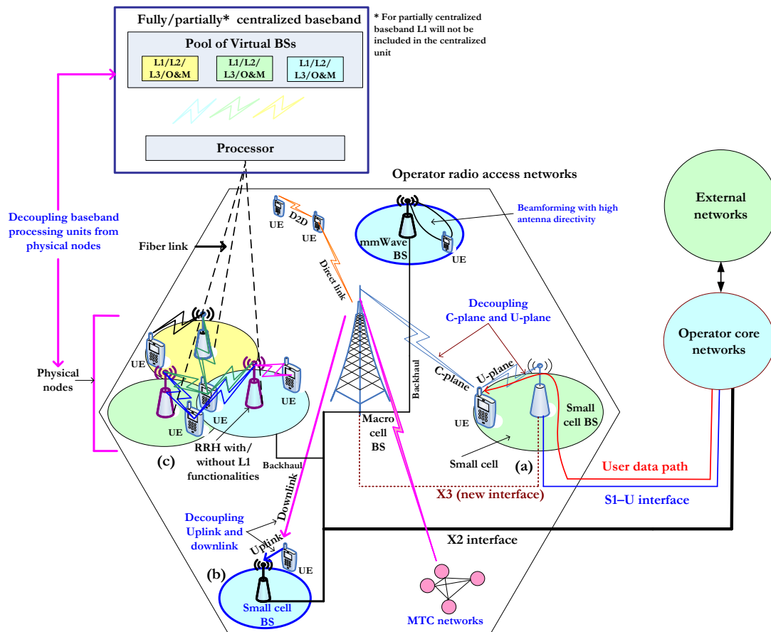
Fig. 6. A device-centric network architectural model for 5G networks.
