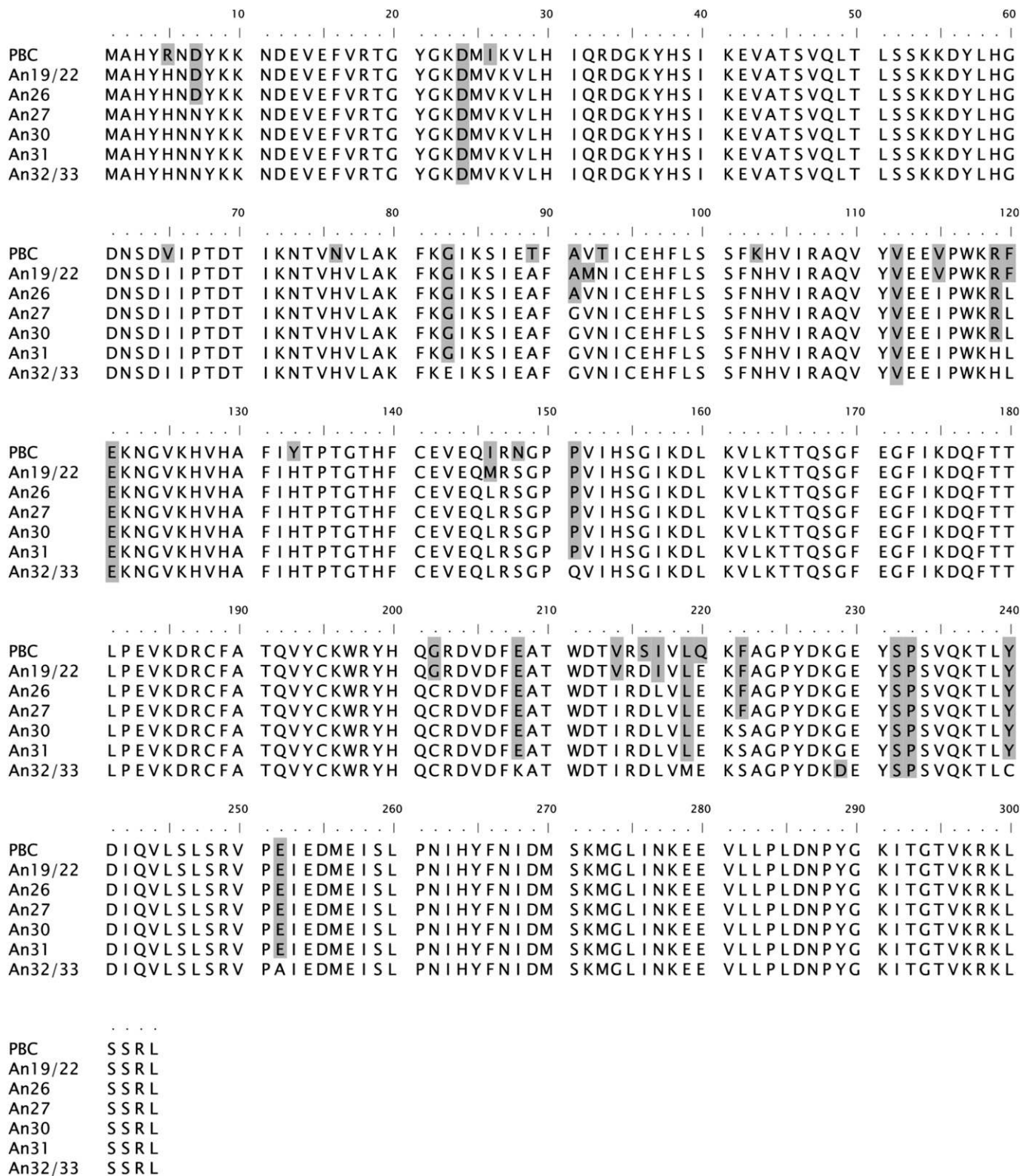
Fig. S5. Ancestral and chimera uricase amino acid sequences. The aligned sequences are labeled according to Fig. 1 in the article and shown in 10-residue blocks. Each sequence is 304 aa long. Also shown is the pig-baboon chimera (PBC) uricase that represents the protein component of the US Food and Drug Administration-approved pegloticase and is included in this alignment for reference. Residues that differ from the human pseudogene are highlighted in gray (except for the two premature stop codons at position 33 and 187).
