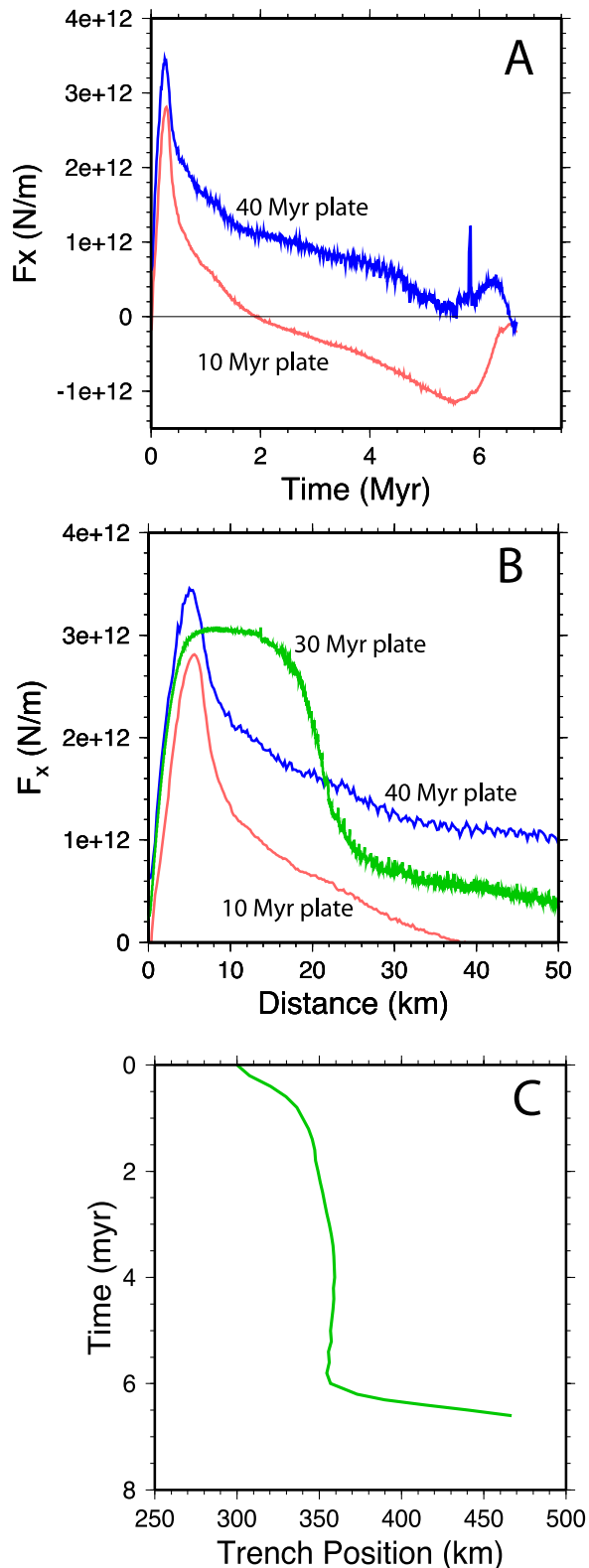
Figure 13. (a) Forces on the edge of the right plate (with an age 40 Myr) and the left plate (with an age of 10 Myr). (b) Force as a function of compression with a homogenesis plate (with an age of 30 Myr) shown for comparison. (c) Position of the trench as function of time since the inception of convergence.
