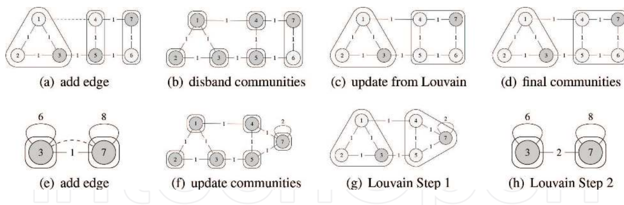
Figure 10. Example of Cordeiro et al. [85] dynamic Louvain for the addition of a cross-community edge (1–4). Top figures show the lower-level network. At the bottom, are shown, the corresponding upper-level network with aggregated communities.
