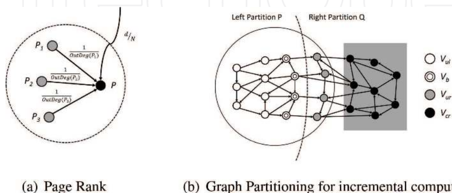
Figure 8. PageRank and graph partitioning used in Desikan et al. [49] incremental page rank.
