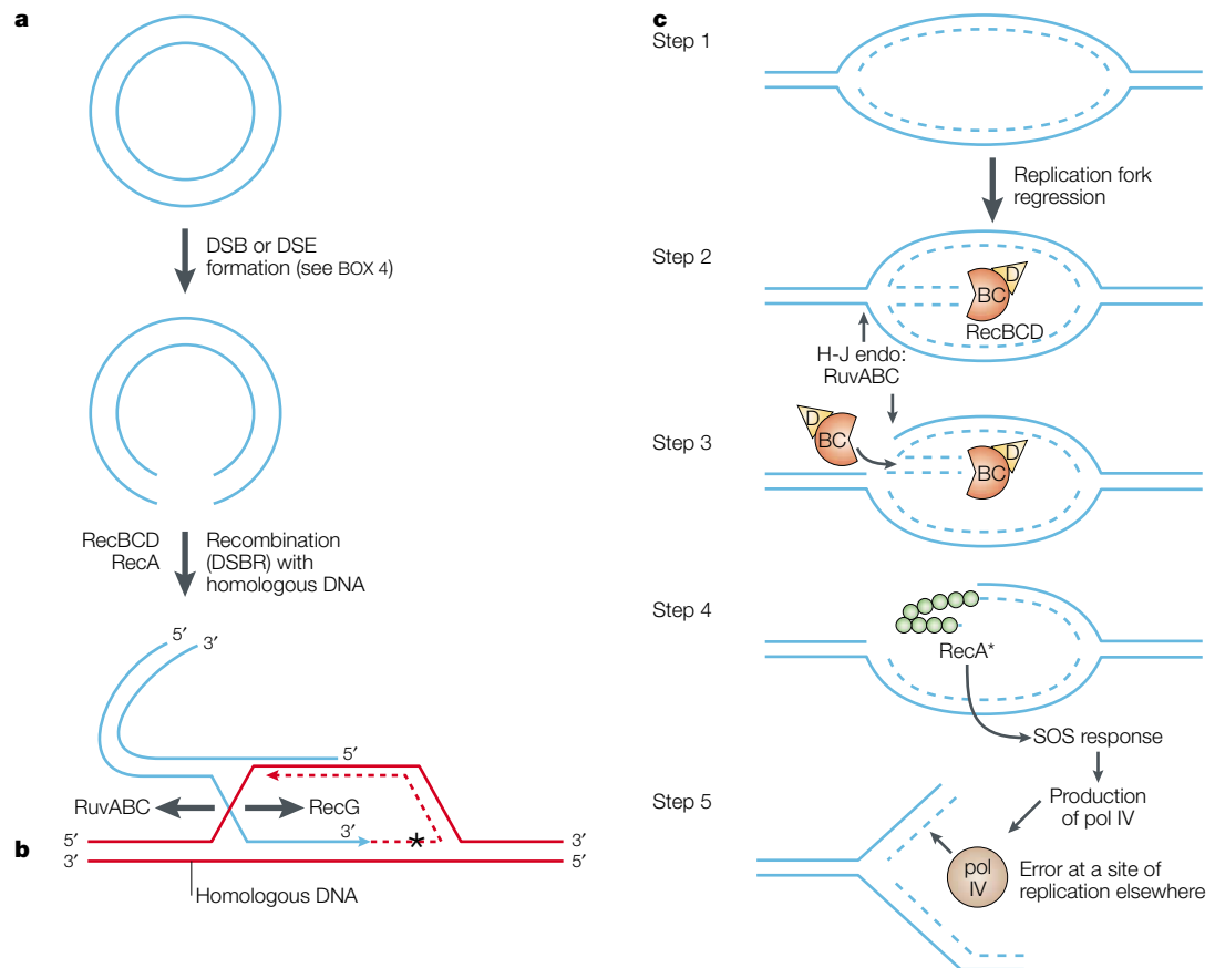
Figure 2 | Two models for generating adaptive point mutations through recombination proteins. Dashed lines represent newly synthesized DNA. a, b | Direct model: replication primed by recombination 39 . In a , the circular F' (or chromosome) acquires a double-stranded break (DSB) or double-stranded end (DSE) by any of the possible ways outlined in BOX 4. DSBR, DSB repair. In b , RecBCD-mediated DSB-repair by homologous recombination allows strand invasion of a region of homologous DNA (perhaps present in a sister chromosome) and primes DNA replication, during which errors accumulate (asterisk). The error could be caused by the mutator DNA polymerase pol IV or by another DNA polymerase. Strand invasion requires RecBC, and RecA, which are required for recombination-dependent adaptive point mutation 39 . The branch migration activity of the RuvABC proteins is proposed to stabilize 3'-end invasion intermediates, which are postulated to prime replication; the opposite polarity branch migration activity of RecG is proposed to unwind and destroy the intermediates that lead to DNA replication 41 . These events might explain the requirement in adaptive point mutation for RuvABC and its depression by RecG 40,41 . DSBs and DSBR are directly associated with mutation in models such as this. In Escherichia coli , the homologous DNA used in recombination could be a sister molecule (present in about 30–40% of stationary-phase cells 124 ), a duplicated region (present in 10 -2 –10 -3 of cells for any given DNA segment 125 ), or even DNA that has been taken up from outside the cell (a process not known to occur in E. coli but that has not been ruled out). c | An indirect model: indirect association of recombination protein action and adaptive point mutation. Step 1, a replication fork stalls. Step 2, regression of the replication fork 120 provides a substrate for RecBCD 39,121 . Step 3, the regressed fork is cleaved by the Holliday-junction endonuclease (H-J endo) activity of RuvABC 39,122 , which is required for adaptive point mutation 40,41 . Step 4, RecA loads onto RecBCD-exposed single strands, leading to activation of the SOS response, production of mutator pol IV and thus (step 5) to error-prone synthesis at some other replication site in DNA, not associated with any direct action of RecA, RecBCD or RuvABC. The SOS response is a DNA damage response in which about 42 DNA repair, recombination and mutation genes are upregulated in response to slowed replication or DNA damage 66 .
