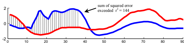
Figure 2: A visual intuition of early abandoning. Once the squared sum of the accumulated gray hatch lines exceeds r^2 , we can be sure the full Euclidean distance exceeds r
