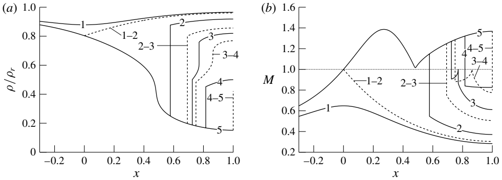
FIGURE 14. Exemplary limiting (----) and intermediate (—) flows of type \mathcal{R}_0^{NC} , computed from the van der Waals polytropic model with c_v/R = 50 . (a) Density solutions, scaled to reservoir density \rho_r ; (b) Mach number solutions. Reservoir conditions: P_r = 1.2315P_c , v_r = 0.7287v_c .
