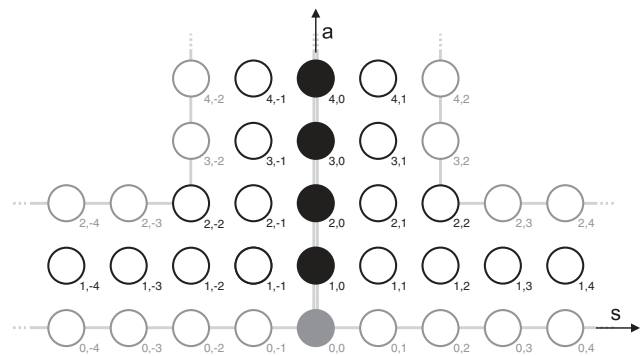
FIG. 1. T-shaped fat hook for the Y and T systems [19]. The middle double line separates the two subgroups with extended SU(2|2)_L and SU(2|2)_R symmetries.
