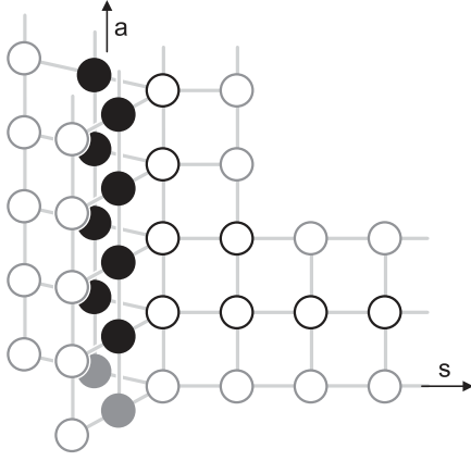
FIG. 2. Fat hook for AdS_4/CFT_3 . The OSP(2, 2|6) symmetry of the ABJM theory, with two momentum carrying nodes, and the SU(2|2) subgroup is manifest in the diagram.
