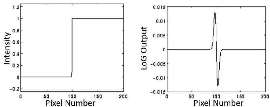
Figure 39: LoG filter response (right) to an intensity step (left) with Gaussian \sigma=3 pixels [42]
