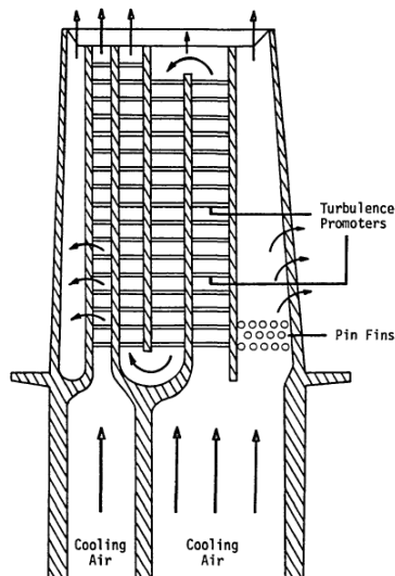
Figure 18: Internal turbine blade cooling [28]
