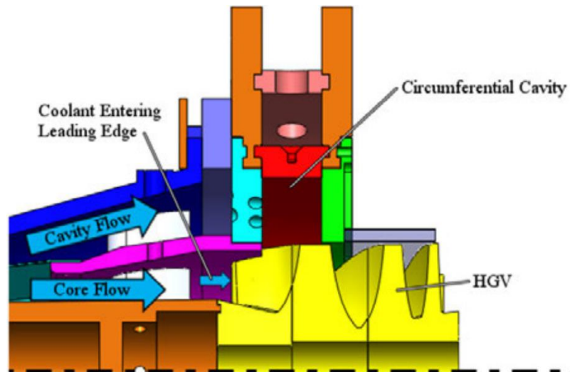
Figure 24: Cross section of AFIT's UCC detailing HGV leading edge location [5]
