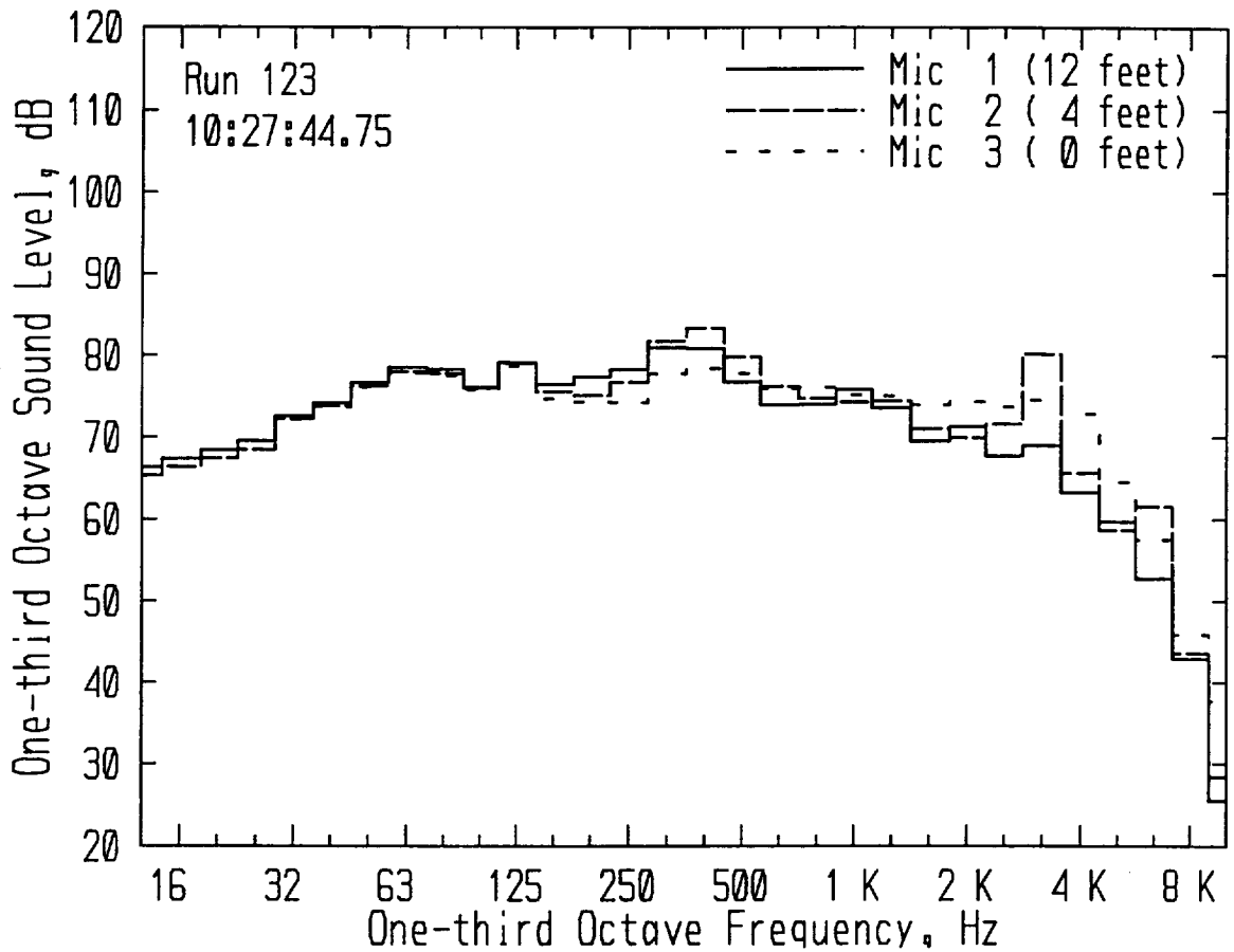
Figure 14. Propagation-adjusted Spectra, Aircraft Height 30 Feet, Distance 666 Feet
