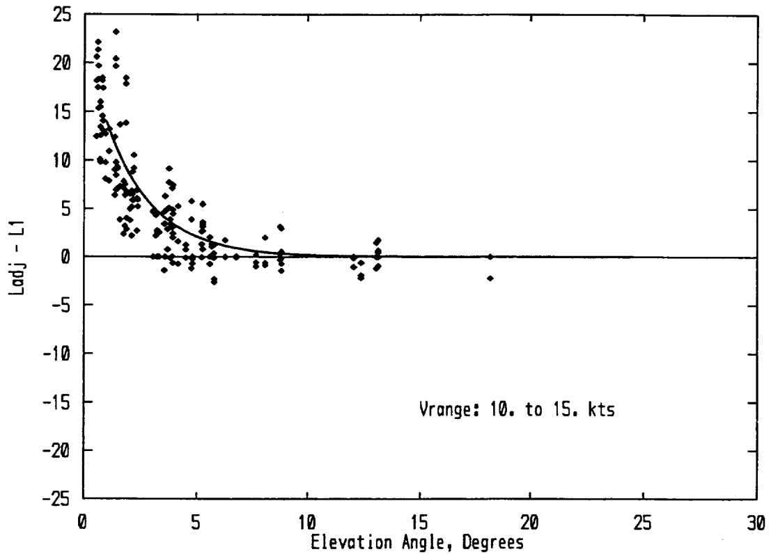
Figure 27. Normalized Noise Levels, Strong Downwind Propagation, EGA Model
