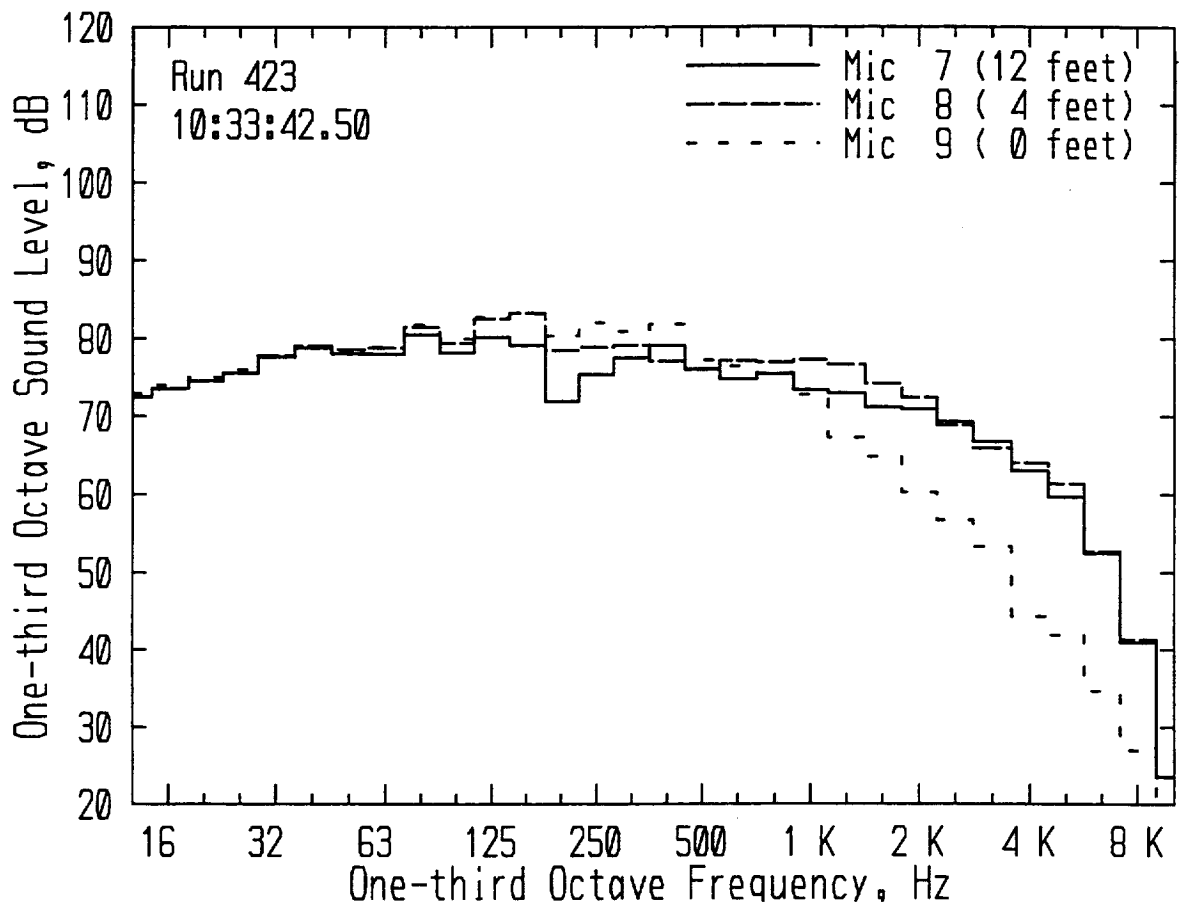
Figure 17. Measured Spectra, Aircraft Height 140 Feet, Distance 1500 Feet
