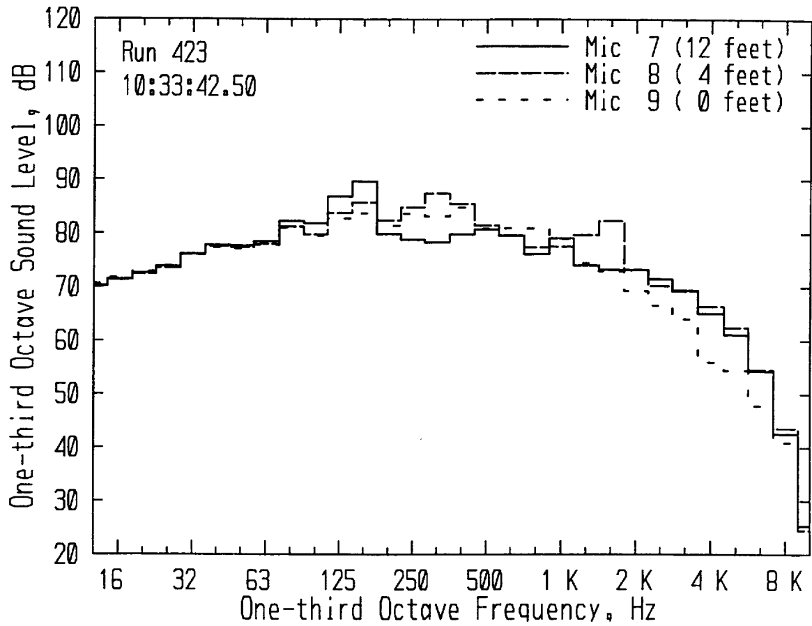
Figure 18. Propagation-adjusted Spectra, Aircraft Height 140 Feet, Distance 1500 Feet
