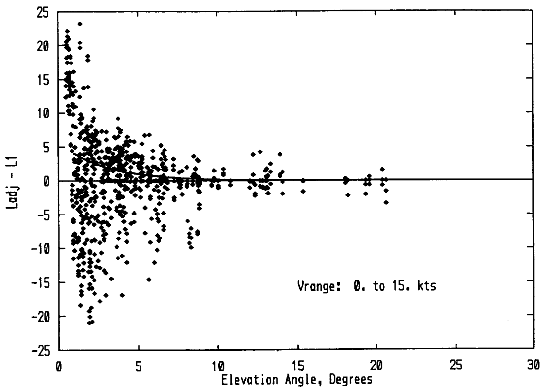
Figure 26. Normalized Noise Levels, Downwind Propagation, EGA Model
