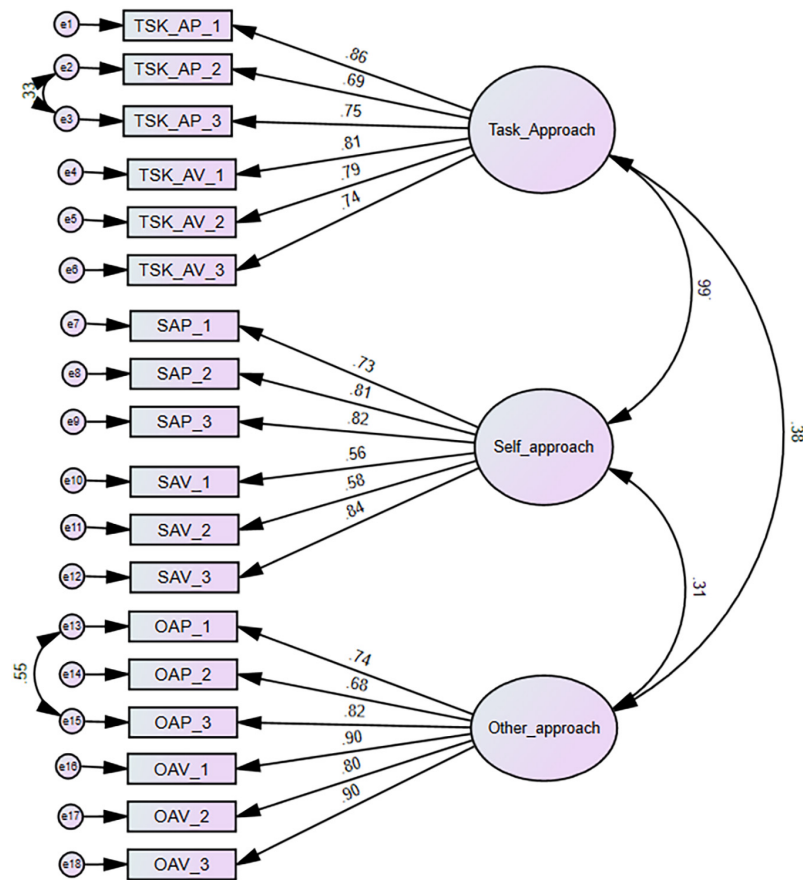
FIGURE 2 | Definition-based AGO model based on EFA result.
