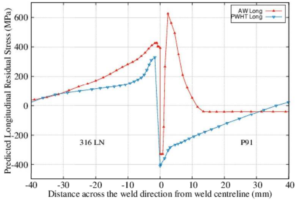
Figure 13. Predicted residual stress across the weld at mid-thickness of the welded plate 95x66mm (300 x 300 DPI)
