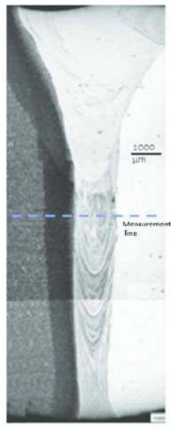
Figure 1. Schematic representation and cross-sectional weld macrograph of the dissimilar metal EB welded specimen
