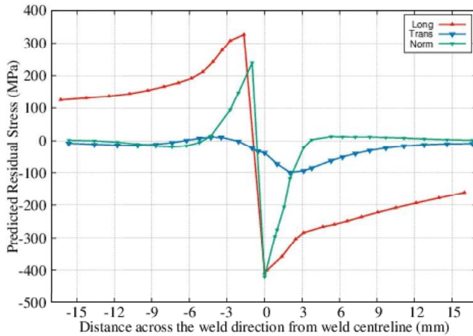
Figure 8. Predicted residual stress across the weld at mid-thickness of the PWHT plate 95x66mm (300 x 300 DPI)
