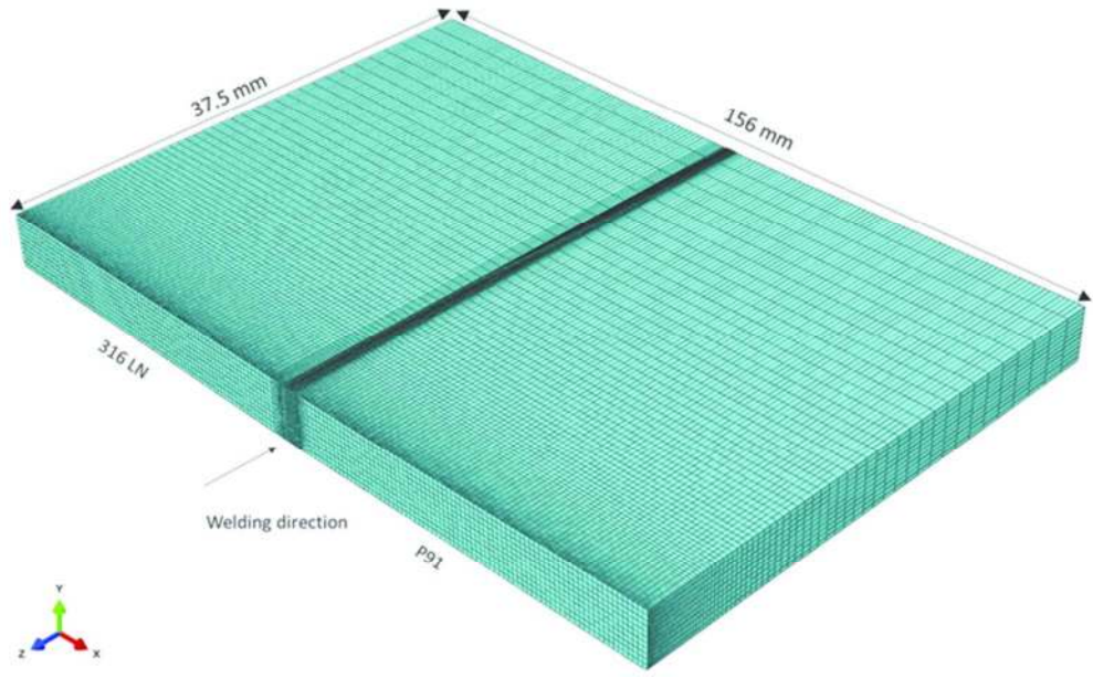
Figure 5. Finite element mesh used for contour measurement 62x38mm (300 x 300 DPI)
