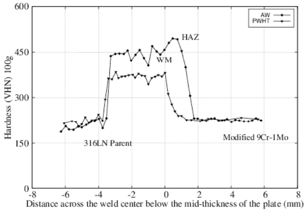
Figure 11. Measured hardness across weld at 1:5mm below the top surface, before and after PWHT
