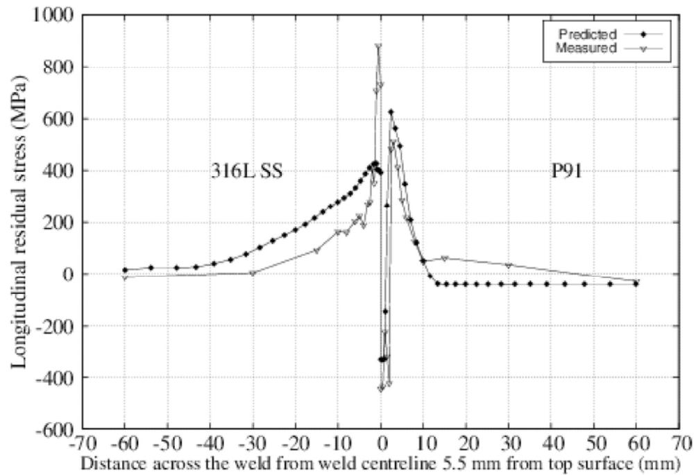
Figure 2. Comparison of predicted and measured residual stresses in the dissimilar welded plate in AW condition across the weld at mid-thickness of the plate
