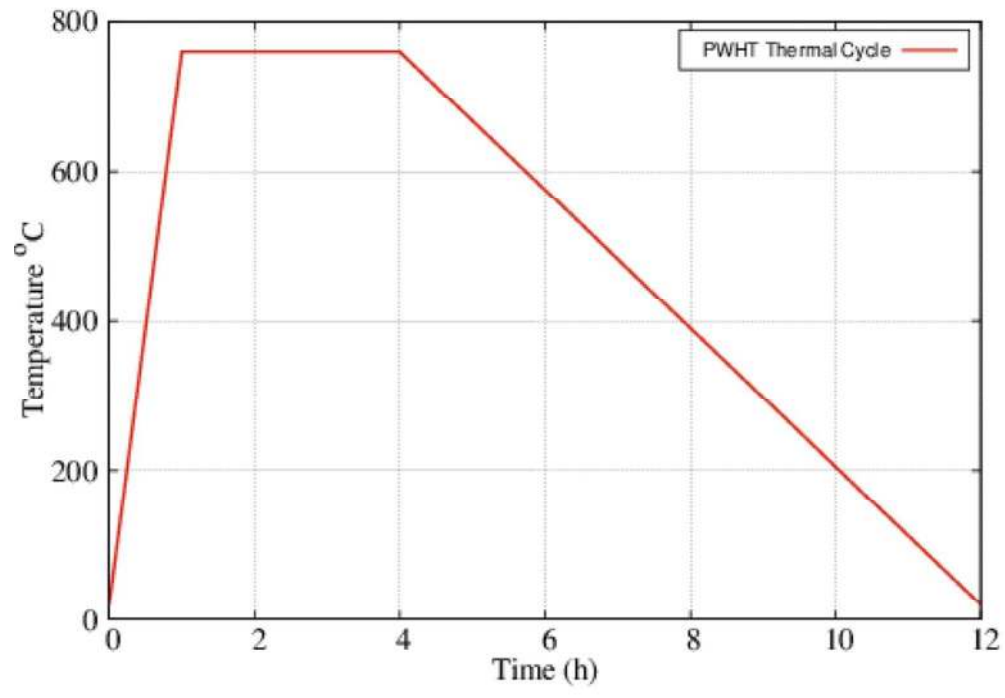
Figure 3. Thermal cycle used in the PWHT simulation
