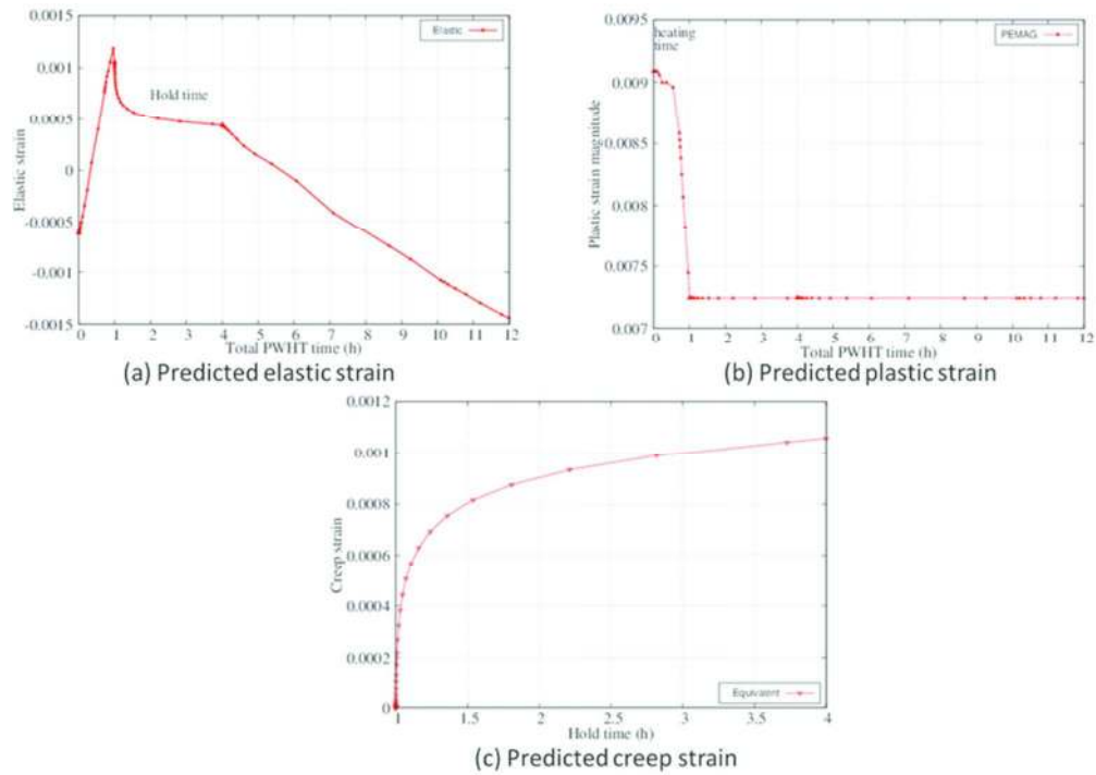
Figure 12. Predicted strain in the weld fusion zone of the welded plate 73x53mm (300 x 300 DPI)
