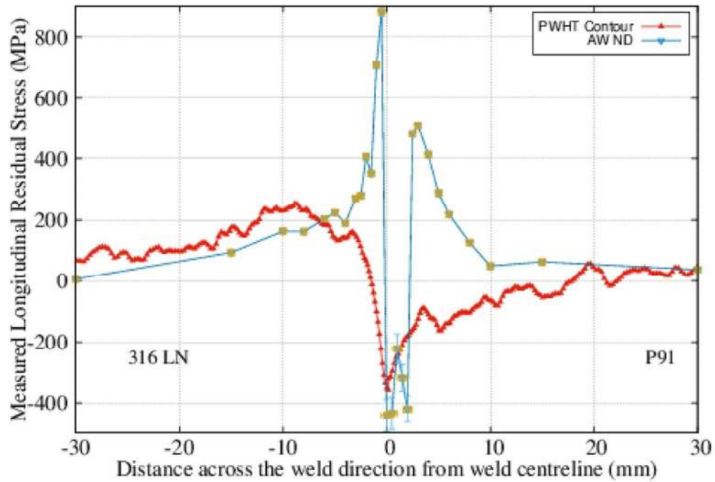
Figure 10. Comparison of the measured residual stress plot across the weld in AW and PWHT condition
