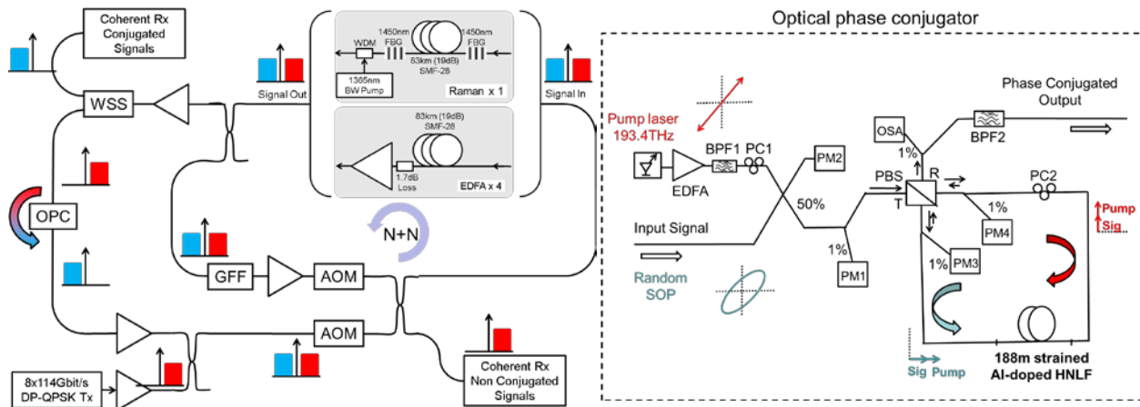
Figure 1. Experimental configuration of (a) the dual input recirculating loop and (b) optical phase conjugator.
