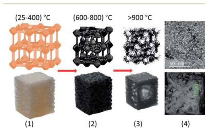
Scheme 1 Schematic illustration for steps in fabricating HPCs from a precursor MOF-5: (1) MOF framework/crystal structure (up to 400 °C) with well-defined pore structure in the micropore region, (2) decomposition, and metal-oxide formation, ZnO and carbon between 600 and 800 °C yielding poor pore development, (3) at >900 °C, ZnO reduction and evaporation of Zn and CO yields highly porous carbon with a hierarchical pore structure and (4) surface morphology of HPCs by TEM & SEM.
