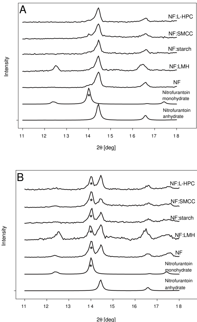
Figure 2. Powder X-ray diffraction patterns of formulations after storage at 85% RH (A) and at 95% RH (B) for 2 weeks. Calculated patterns of nitrofurantoin anhydrate and nitrofurantoin monohydrate are shown as controls. Formulations containing nitrofurantoin anhydrate (NF), NF:LMH, NF:starch, NF:SMCC, and NF:L-HPC. * indicates characteristic peaks of nitrofurantoin monohydrate.
