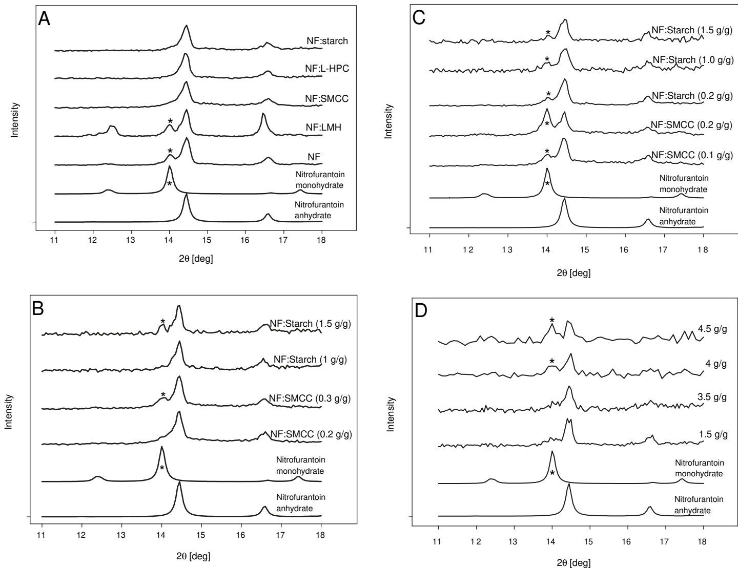
Figure 4. (A) XRPD patterns of nitrofurantoin wet masses after water addition of 0.1 g/g into the formulation on the first day. Formulations with nitrofurantoin anhydrate (NF):LMH, NF:SMCC, NF:L-HPC, and NF:starch measured in the angular range of 11 to 18°2 \theta . (B) XRPD patterns of nitrofurantoin wet masses after different water additions into the formulation on the first day. Formulations with SMCC (water additions of 0.2 or 0.3 g/g) and starch (water additions of 1 or 1.5 g/g) measured in the angular range of 11 to 18° 2 \theta . (C) XRPD patterns of nitrofurantoin wet masses after different water additions into the formulation on the second day. Formulations with SMCC (water additions of 0.1 or 0.2 g/g) and starch (water additions of 0.2, 1, or 1.5 g/g) measured in the angular range of 11 to 18°2 \theta . (D) XRPD patterns of nitrofurantoin wet masses containing L-HPC (1:1) on the second day. Water additions of 1.5, 3.5, 4, or 4.5 g/g into the formulation measured in the angular range of 11 to 18° 2 \theta .
