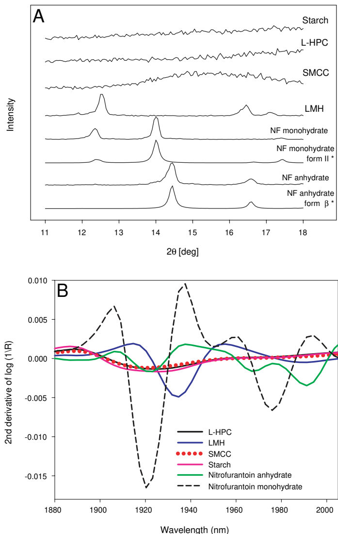
Figure 1. (A) Powder X-ray diffraction patterns of nitrofurantoin anhydrate (NF anhydrate), nitrofurantoin monohydrate (NF monohydrate) and studied excipients: LMH, SMCC, L-HPC (grade LH-21), and modified starch in the angular range of 11 to 18° 2 \theta . * indicates calculated XRPD patterns of nitrofurantoin anhydrate (NF anhydrate form \beta ) and nitrofurantoin monohydrate (NF monohydrate form II), shown as controls. (B) NIR reflectance spectra of 4 excipients and spectra of nitrofurantoin anhydrate and monohydrate as controls. The second derivative of absorbance, \log(1/R) , at 1,880 to 2,005 nm. Characteristic peaks of nitrofurantoin monohydrate are shown at 1,920 and 1,975 nm.
