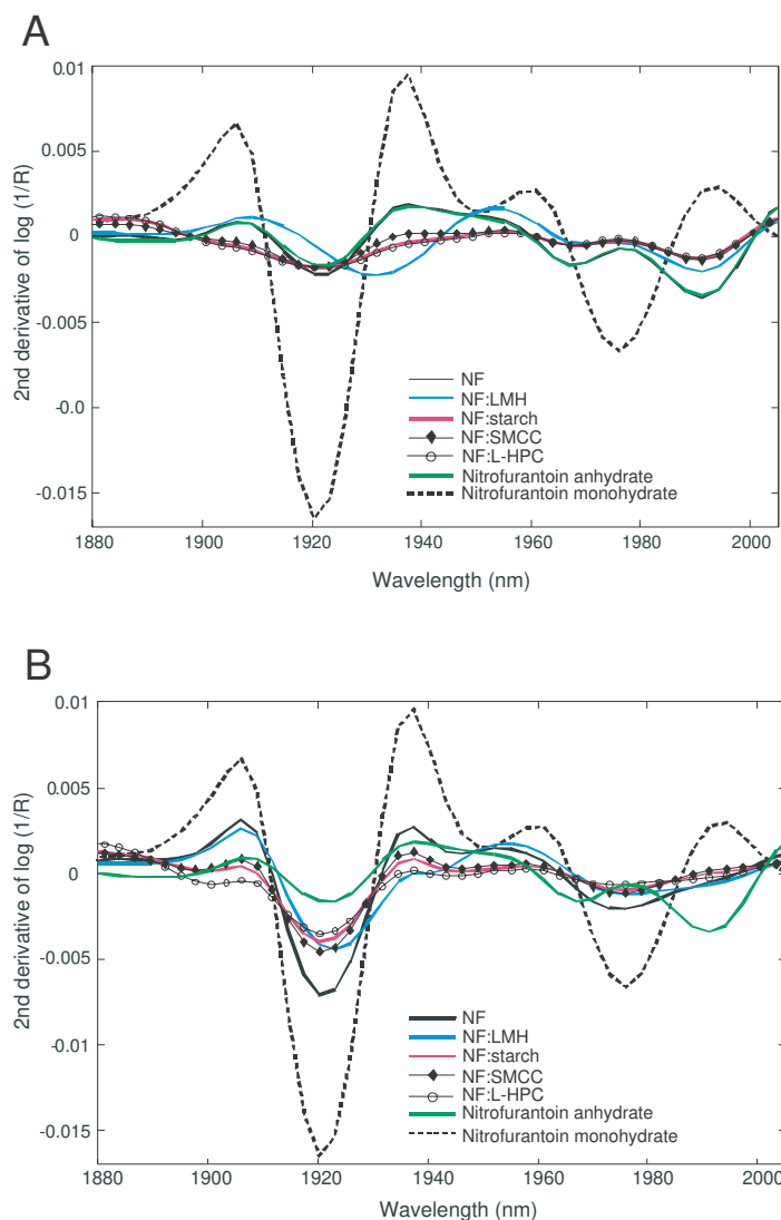
Figure 3. NIR reflectance spectra of formulations after storage at 85% RH (A) and at 95% RH (B) for 2 weeks. The second derivative of absorbance, \log(1/R) , at 1,880 to 2,005 nm. Formulations containing nitrofurantoin anhydrate (NF), NF:LMH, NF:starch, NF:SMCC, and NF:L-HPC. Nitrofurantoin anhydrate and nitrofurantoin monohydrate are shown as controls. Characteristic peaks of nitrofurantoin monohydrate are shown at 1,920 and 1,975 nm.
