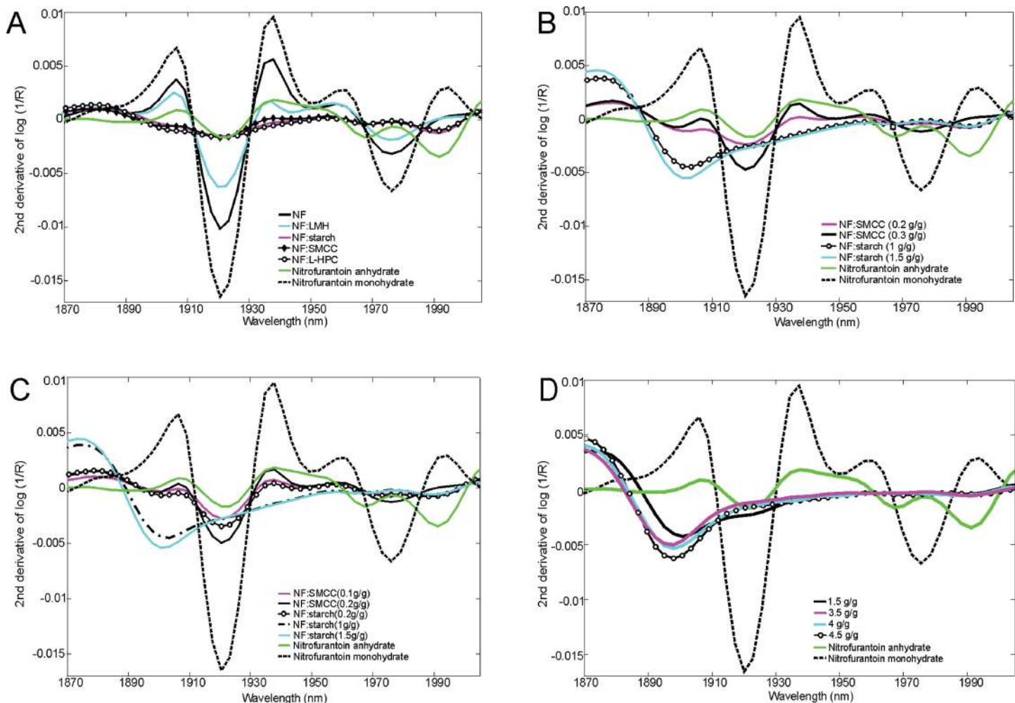
Figure 5. (A) Second-derivative NIR spectra of nitrofurantoin wet masses after water addition of 0.1 g/g into the formulation on the first day. Formulations (1:1) containing nitrofurantoin anhydrate (NF):LMH, NF:SMCC, NF:L-HPC, and NF:starch. The second derivative of absorbance, \log(1/R) , at 1,870 to 2,005 nm. Characteristic peaks of nitrofurantoin monohydrate are shown at 1,920 and 1,975 nm. (B) Second-derivative NIR spectra of nitrofurantoin wet masses after different water additions into the formulation on the first day. Formulations (1:1) containing SMCC (water additions of 0.2 or 0.3 g/g) and starch (water additions of 1 or 1.5 g/g) at 1,870 to 2,005 nm. (C) Second-derivative NIR spectra of nitrofurantoin wet masses after different water additions into the formulation on the second day at 1,870 to 2,005 nm. Formulations containing SMCC (water additions of 0.1 or 0.2 g/g) or starch (water additions of 0.2, 1 or 1.5 g/g). (D) Second-derivative NIR spectra of nitrofurantoin wet masses containing L-HPC (1:1) on the second day at 1,870 to 2,005 nm. Water additions of 1.5, 3.5, 4, or 4.5 g/g into the formulation.
