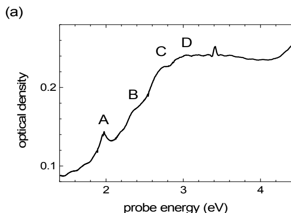
Figure 1. Extinction spectrum of few-layer WS 2 in PMMA. The different exciton absorption resonances are labeled from A to D.
