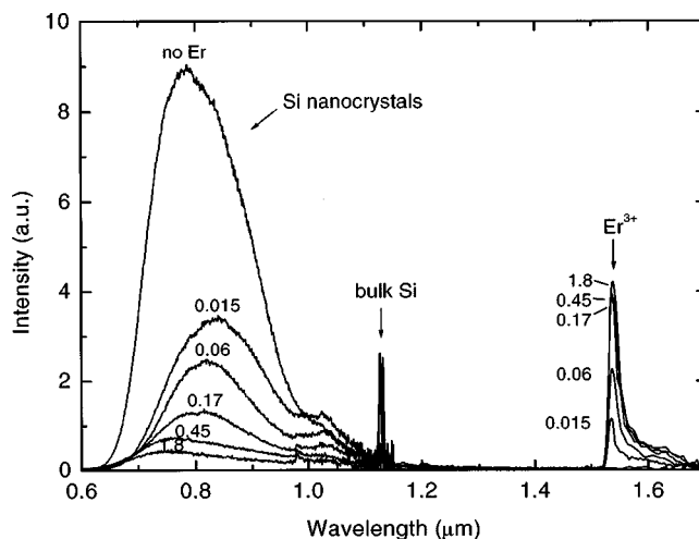
FIG. 2. Photoluminescence spectra of Si nanocrystal-doped \text{SiO}_2 containing different Er concentrations in the range of 0–1.8 at. %, measured at 15 K using a pump power of 1 mW at 458 nm.
