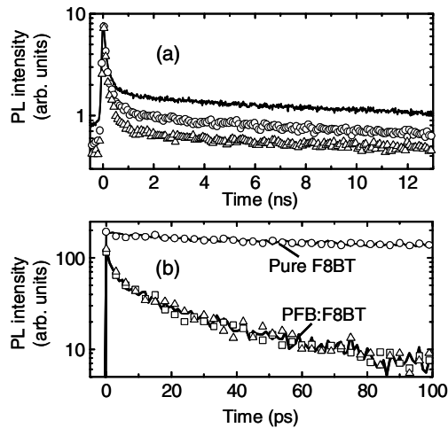
FIG. 3. (a) Photoluminescence decay measured using TCSPC (excitation: 407 nm, <4 nJ/cm 2 ; detection: 640 nm) from a PFB:F8BT device at room temperature under 0 V (continuous line), 13 V (circles), and 30 V (triangles) applied reverse biases. (b) PLUC measurements (excitation: 405 nm, 42 nJ/cm 2 ; detection: 550 nm) from a similar device at 0 V (continuous line), 5 V (squares), and 12.5 V (triangles) reverse bias. For comparison, data for a device with pure F8BT at 0 V (continuous line) and 12 V (circles) are also plotted.
