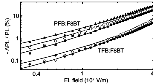
FIG. 4. Relative electric field quenching of the PFB:F8BT and TFB:F8BT exciplex photoluminescence intensities (measured at 700 and 580 nm, respectively), in the same devices as in Fig. 2, versus electric field at 230 K (solid squares), 250 K (open and solid circles), 290 K (solid triangles), and 295 K (open diamonds). The solid lines through the data are Onsager simulations (parameters for PFB:F8BT: \epsilon = 3.5 , r_{gp} = 3.0 nm at T = 230 K and 3.1 nm at 250 and 290 K; for TFB:F8BT: \epsilon = 3.5 , r_{gp} = 2.3 nm at T = 250 K and 2.2 nm at 295 K).
