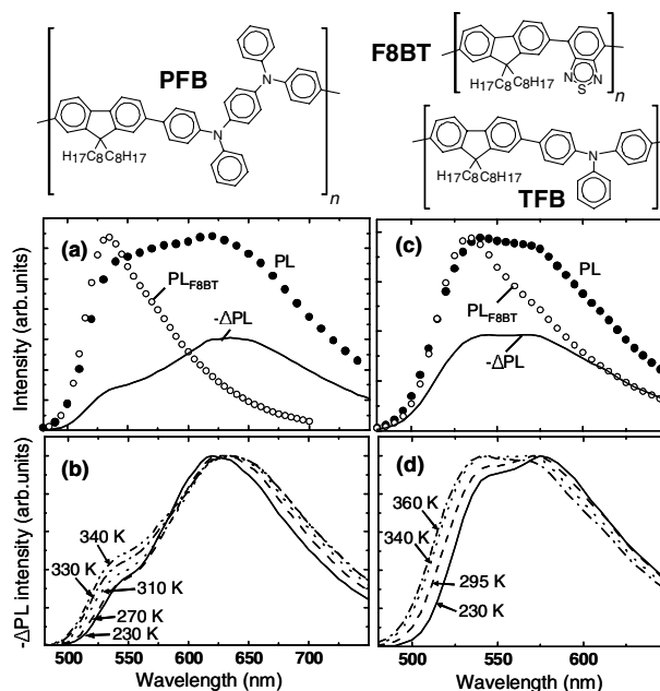
FIG. 2. (a) Photoluminescence intensity (PL, solid circles) and reduction of photoluminescence intensity due to an applied reverse bias of 10 V ( \Delta PL , continuous line) for a PFB:F8BT blend device at 340 K. PL and -\Delta PL are plotted in the same scale and reflect their relative intensities. (b) \Delta PL spectra (at 10 V) from the same device as in (a) at different temperatures. (c) PL (solid circles) and \Delta PL at a reverse bias of 15 V (continuous line) for a TFB:F8BT blend device at 340 K. (d) \Delta PL spectra from the same device as in (c) at different temperatures. For comparison, the PL spectrum from an F8BT-only device (open circles) is plotted in both parts (a) and (c). The structures of PFB, F8BT, and TFB are also shown.
