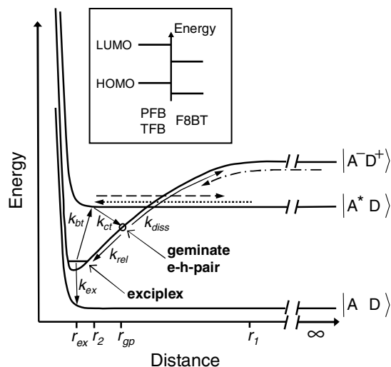
FIG. 1. Potential energy diagram describing the energetics and kinetics at type II polymer heterojunctions. The energetic order of |A^-D^+\rangle_{r=\infty} and |A^*D\rangle_{r=\infty} may be reversed for PFB:F8BT vs TFB:F8BT. The inset shows the band offsets at a type II heterojunction (see also [7]).
