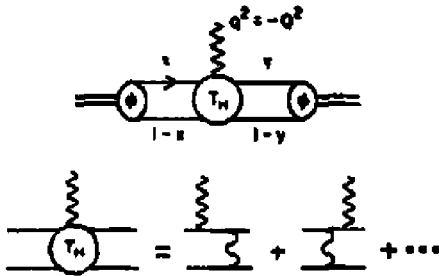
Fig. 2. Factorized structure and leading QCD contributions for the pion form factor in QCD.
