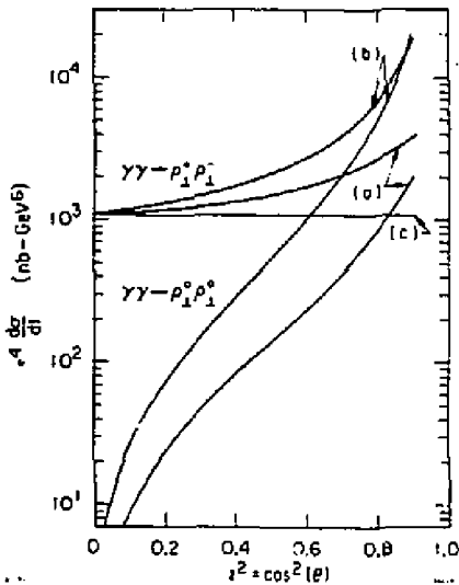
Fig. 7. QCD predictions for \gamma\gamma \rightarrow \rho_1 \rho_1 with opposite helicity \pm 1 to leading order in QCD. The normalization given here assumes that the \rho distribution amplitude is helicity independent.
