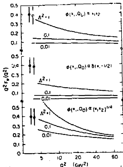
Fig. 3. Leading order QCD predictions for the pion form factor assuming various distribution amplitudes \phi(x_1, Q_0) at Q_0^2 = 2 \text{ GeV}^2 and various values of the QCD scale parameter \Lambda^2 . The data are from the analysis of electroproduction e^-p \rightarrow e^- + \pi^+ + n ; C. Bebek et al. , Ref. 41.
