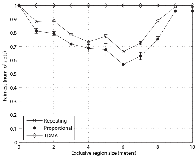
Fig. 5. Fairness comparisons w.r.t. number of slots, Nakagami- m=4 . The error bars represent 95% confidence interval.
