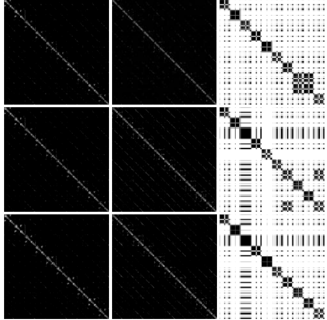
Figure 4. From left to right: The columns are the visualization of subspace representations Z_1 , Z_2 and the indicator matrix \Theta , respectively. From top to bottom: The rows are the results of ECMSC _{\alpha=0} (ACC = 0.701), ECMSC _{\beta=0} (ACC = 0.689) and ECMSC (ACC = 0.781), respectively.
