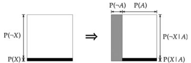
Figure 1. Meta-level uncertainty.
