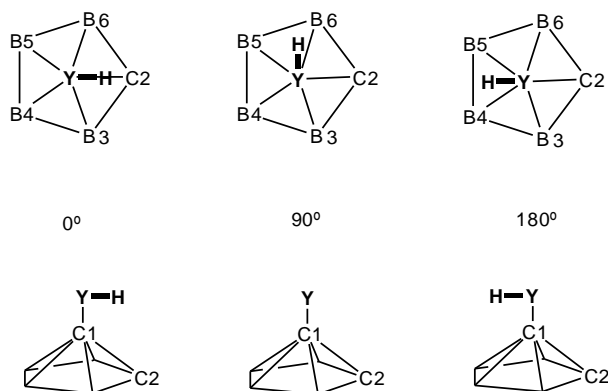
Figure 10. Bond length (Å) and relative energy (kJmol -1 ) data for MP2/6-31G* optimised geometries for model compounds HCb 0 X. The torsion angles C2-C1-Y/Z-H in these model compounds were fixed at 0°, 90° or 180°.
