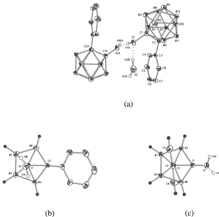
Figure 2. Structure of the hemihydrate \text{PhCb}^{\circ}\text{OH}\cdot 0.5\text{H}_2\text{O} . (a) hydrogen bonding interactions (only one disorder component is shown); distances( \text{\AA} ) and angles( ^{\circ} ), \text{O1}\cdots\text{H2B} 2.11, \text{O1A}\cdots\text{H1A} 1.98, \text{O1}\cdots\text{O1A} 2.78, \text{O1}\cdots\text{O2} 2.72, \text{O1}\cdots\text{H2B}-\text{O2} 133, \text{O1A}\cdots\text{H1A}-\text{O1} 174; (b) view down the exo OC bond; (c) view down the exo PhC bond
