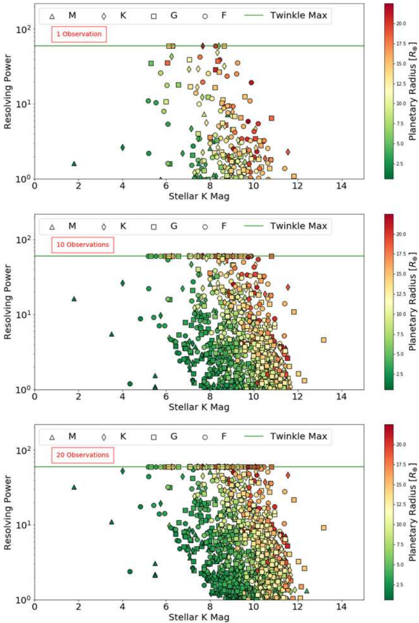
Fig. 16 Achievable resolving power in the second infrared channel (2.42 – 4.5 μm) for currently-known exoplanets and predicted TESS planets within Twinkle’s field of regard assuming a requirement of SNR ≥ 7 for a given number of transit or eclipse observations. The colour of the point indicates the planetary radius, the shape indicates the stellar type of the host star and the green line represents Twinkle’s maximum resolving power in the channel
