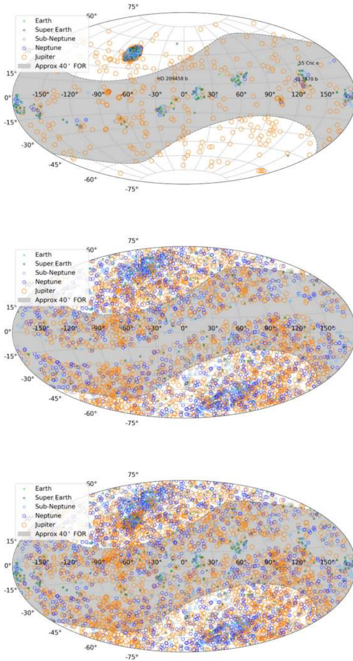
Fig. 3 Top: Currently-known transiting exoplanets, their planetary classification and the sweep of Tinsdale's field of regard. The initial Kepler field is the densely populated region at RA -70^\circ , Dec 45^\circ and the locations of some well-known exoplanets are noted. Middle: Predicted TESS planet detections. Bottom: Currently-known planets and predicted TESS detections
