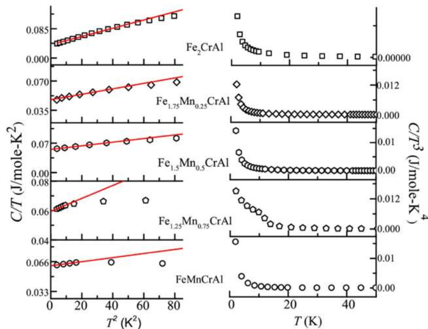
Figure 5. Left panel: C/T vs. T^2 plot of all the alloys and fitted (solid red line) with Eq. 4. Right panel: C/T^3 vs. T plot of all the alloys.
