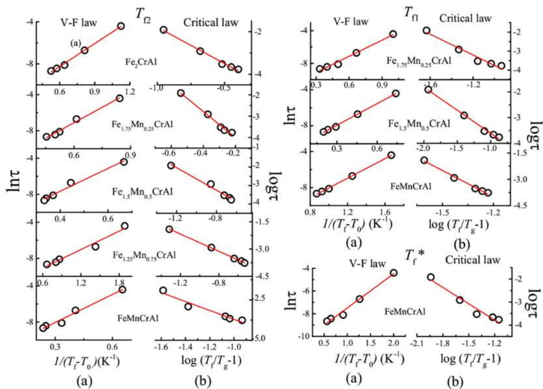
Figure 8. (a) V-F law fit of relaxation time ( \tau ) as function of reduced temperature 1/(T_f - T_0) using Eq. 7 (b) Critical law fit of relaxation time ( \tau ) as function of reduced temperature (T_f/T_g - 1) using Eq. 6 for T_f^* , T_{f1} and T_{f2} for respective alloys.
