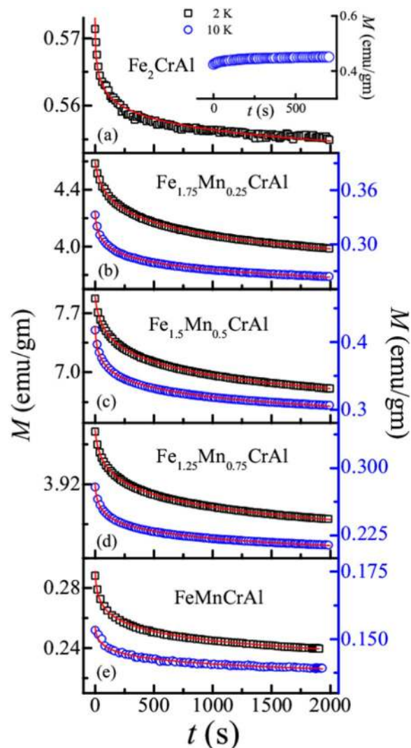
Figure 4. (a–e) Magnetization as a function of time at different temperature for all the alloys. Inset of (a) represents the relaxation behaviour of \text{Fe}_2\text{CrAl} at 10 K. Solid red line depicts the logarithmic fit using Eq. 3. Note: Left axis represents the scale for data obtained at 2 K and right axis represents the scale for the data obtained at 10 K.
