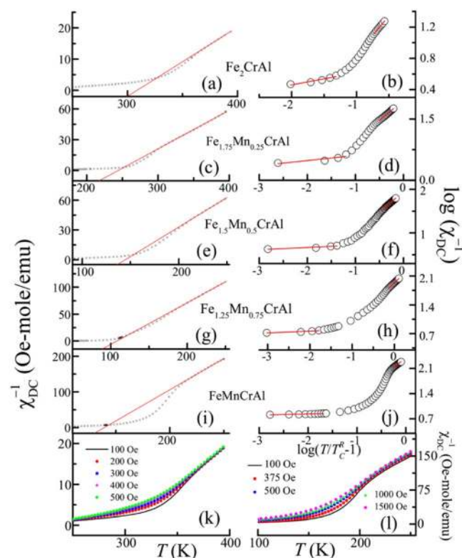
Figure 11. Left panel: (a,c,e,g,i) represent Inverse DC susceptibility as function of temperature plot at 100 Oe. Solid red line represents the fitting using CW law. Right panel: (b,d,f,h,j) represent the log-log plot of \chi_{DC}^{-1} vs. T/T_C^R - 1 . Solid red lines are straight line fitting in GP and PM region. (k,l) depicts Inverse DC susceptibility as function of temperature plot at different applied fields for Fe_2CrAl and FeMnCrAl respectively.
