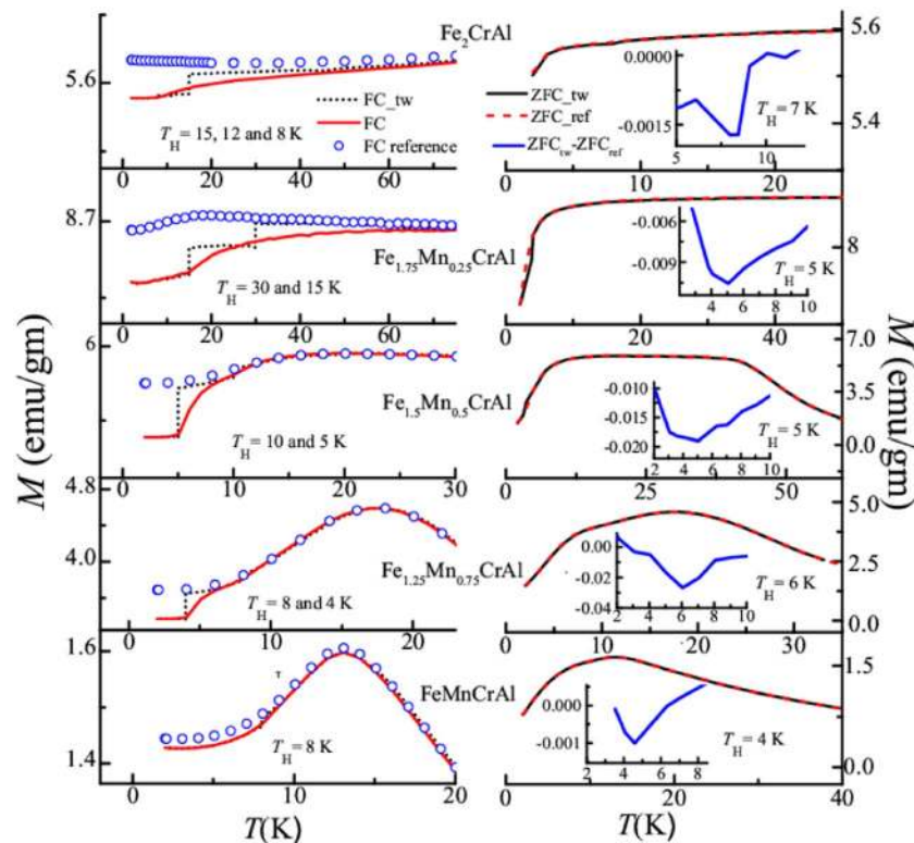
Figure 6. Temperature dependent memory effect of all the alloys at different halt temperatures ( T_H ); Left panel: Under FC condition. Right panel: Under ZFC condition. Insets of right panel: Temperature response of ZFC_{tw} - ZFC_{ref} .
