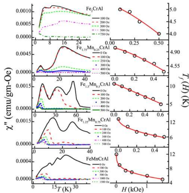
Figure 9. Left panel: Temperature response of out-of phase component of AC susceptibility at different H_{DC} . Right panel: T_f vs. H plot obtained from out-of-phase component of AC susceptibility and fitted (solid red line) with Eq. 8.
