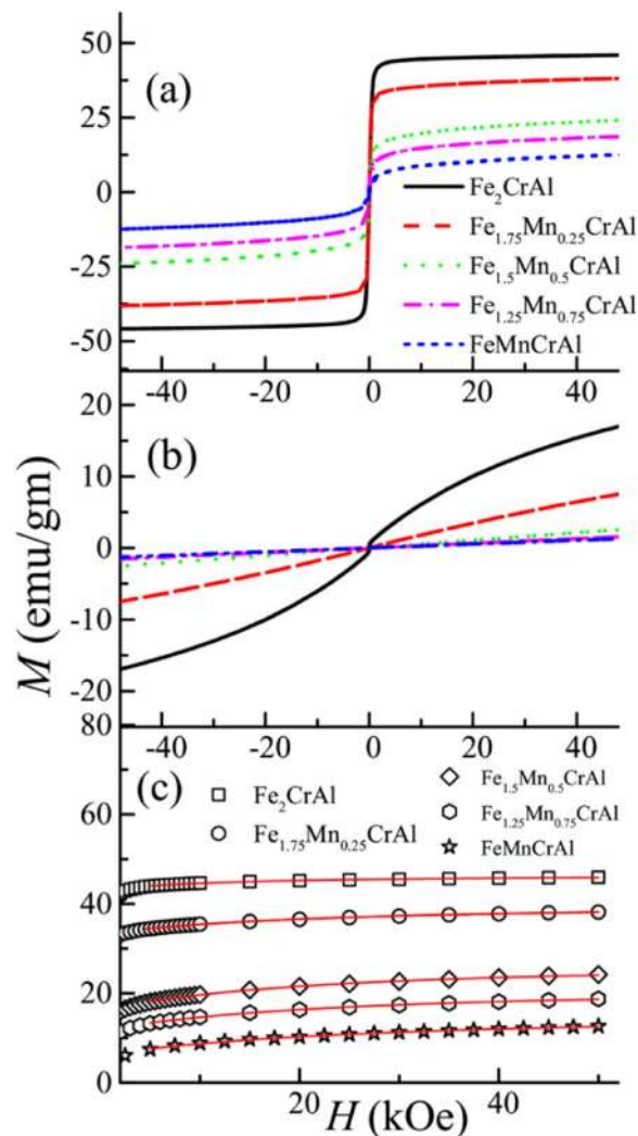
Figure 3. Isothermal magnetization as a function of magnetic field at (a) 2 K and (b) 300 K of \text{Fe}_{2-x}\text{Mn}_x\text{CrAl} ( x \leq 1 ) alloys (c) Magnetic field dependent magnetization plots of all alloys at 2 K with fit (red solid line) using Eq. 2.
