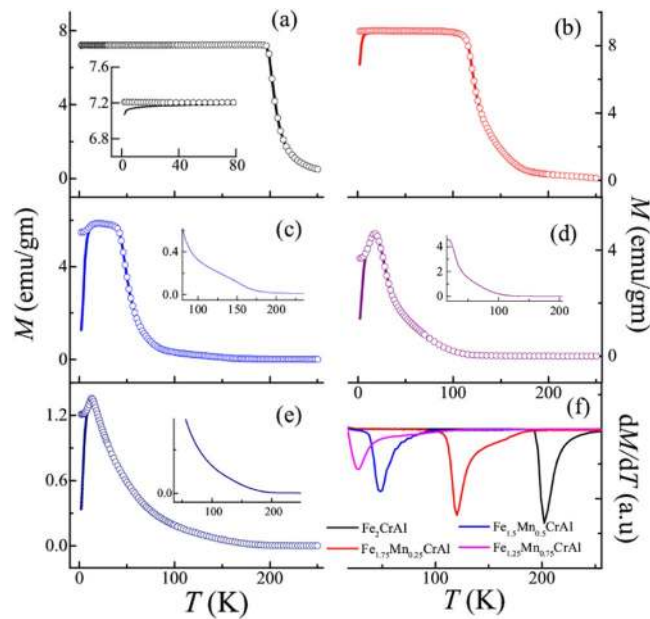
Figure 2. Temperature response of the DC magnetization under ZFC (straight line) and FC (open circle) conditions at 100 Oe in the temperature range 2–250 K for (a) \text{Fe}_2\text{CrAl} . (b) \text{Fe}_{1.75}\text{Mn}_{0.25}\text{CrAl} (c) \text{Fe}_{1.5}\text{Mn}_{0.5}\text{CrAl} ; (d) \text{Fe}_{1.25}\text{Mn}_{0.75}\text{CrAl} ; (e) \text{FeMnCrAl} . Inset of (a) shows the magnified view of ZFC and FC curves in the temperature range 2–80 K, while, insets of (c–e) shows magnified view of the respective ZFC curves (f) dM/dT vs T plot for \text{Fe}_{2-x}\text{Mn}_x\text{CrAl} ( x \leq 0 < 1 ) alloys in the temperature range 18–250 K.
