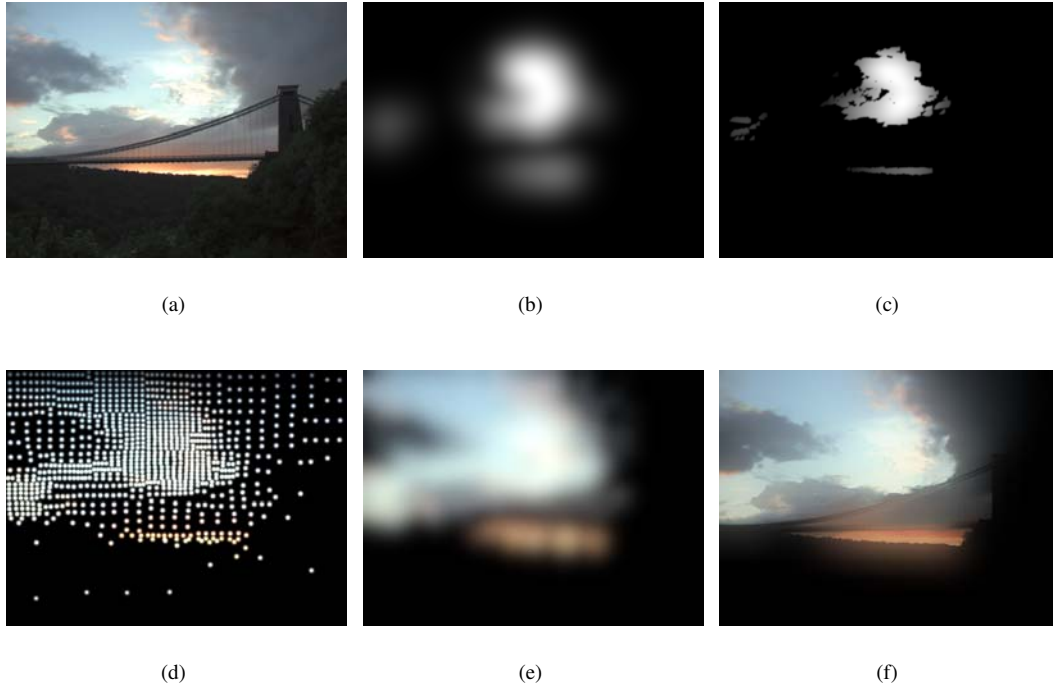
Figure 4: A comparison between methods for generating the expand map. In the top row the method presented in [Rempel et al. 2007]: a) A single exposure LDR image. b) Gaussian filtered of thresholded luminance for a). c) The final expand map with the application of an edge stopping function to b). In the bottom row our method: d) Light source samples for a) generated using median cut algorithm. e) The expand map, for each color channel, which is the result of the density estimation applied to d). f) Final expand map for a) applying cross/joint bilateral filter to e) using luminance of a) as guidance.
