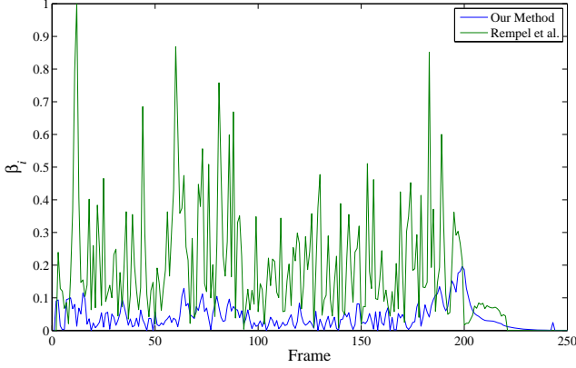
Figure 8: The graph for values of \beta_i for each frame for the sequence fireball-smoke.avi. Our method compared to R . present less fluctuations and of lower intensity.
