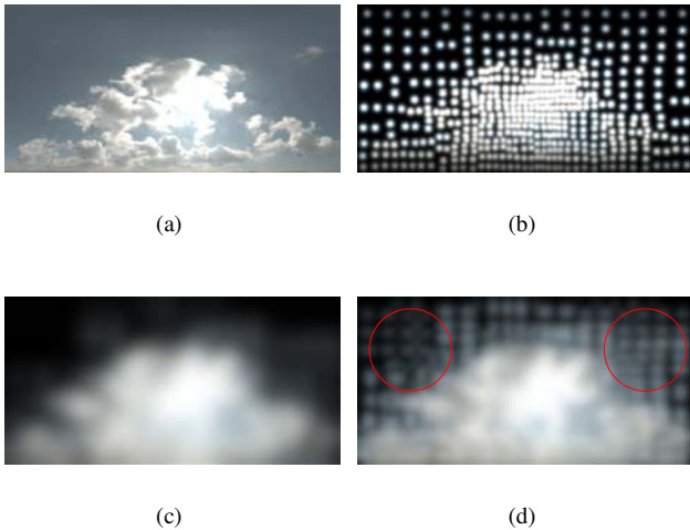
Figure 5: A comparison between automatic and non automatic density estimation for the 20-th frame of the sky sequence: a) The LDR frame. b) The light sources generated by median cut. c) The result of the density estimation using automatic parameters estimation. d) The result of the density estimation using parameters which were estimated by a user for the first frame. Note inside red circles the expand map is estimating wrongly the density of light sources generating areas to expand.
