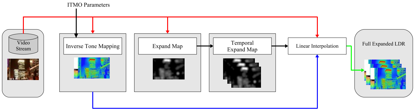
Figure 2: The inverse tone mapping pipeline.
