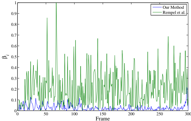
Figure 7: The graph for values of \beta_i for each frame for the sequence fireball.avi. Our method compared to \mathbf{R} . present less fluctuations and of lower intensity.
