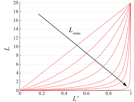
Figure 3: iTMO curves, showing how L_{\text{white}} is related to the shape of the iTMO. In this example different curves are plotted with an increasing value for L_{\text{white}} 1, 2.5, 5, 10, 25, 50, 100, and 1000 (the arrow shows the increasing direction).
