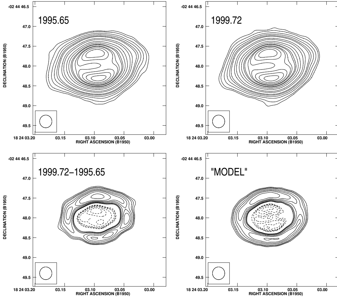
Fig. 1. Top: contour images of the 3.6 cm continuum emission from M2-43 for 1995.65 (left) and 1999.72 (right). The contours are -4, 4, 8, 20, 40, 70, 100, 200, 300, 500, 700, 900, 1000, 1100, 1200, 1300, 1500, 1700, and 1900 times 14 \mu\text{Jy beam}^{-1} , the average rms noise of the images. Bottom: contours of the 3.6 cm difference image (left) and of the “model” (right) obtained as described in the text. The contours are -12, -10, -8, -6, -5, -4, 4, 5, 6, 8, 10, 12, 15, and 20 times 20 \mu\text{Jy beam}^{-1} , the rms noise of the difference image. The restoring beam ( 0''.32 \times 0''.31 with a position angle of 0^\circ ) is shown in the bottom left corner of each image.
