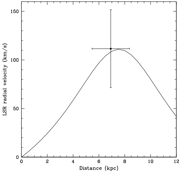
Fig. 2. In this figure we show (solid line) the expected LSR radial velocity as a function of distance to the Sun in the direction of M2-43 for the galactic rotation model of Brand & Blitz (1993). The point marks the estimated distance and the observed LSR radial velocity for M2-43.
