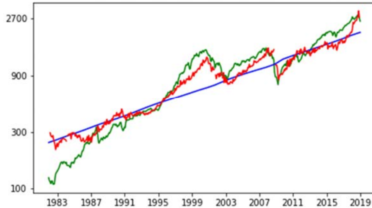
Figure 2. We plot in logscale the levels of the S&P500 index (green line), the rational benchmark index ( p_t^{RE} , blue line, footnote 10), and the price index based on earnings forecasts ( \tilde{p}_t , red line, Equation 4).
