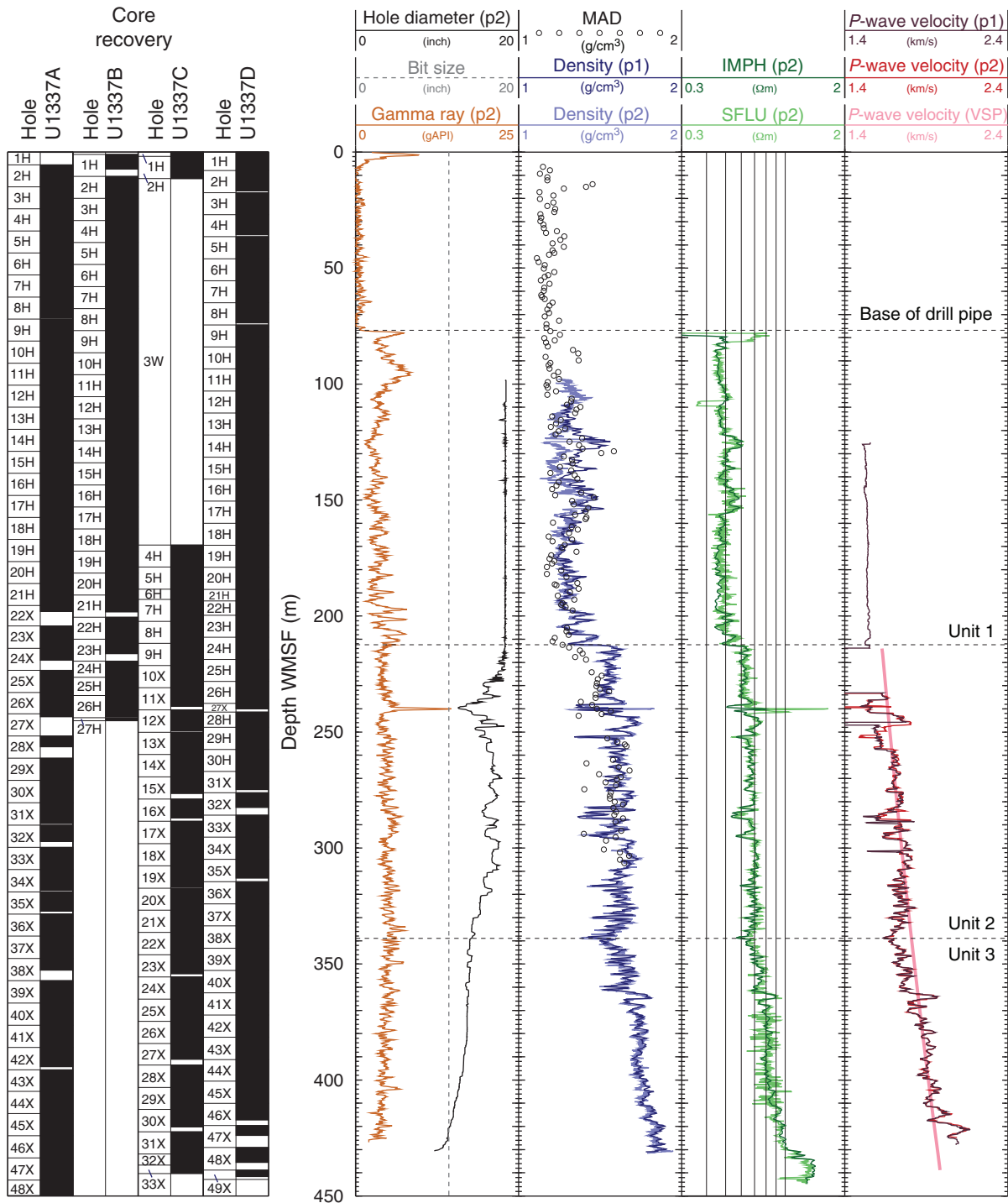
Figure F77. Downhole log measurement summary, Hole U1337A. p1 = uplog Pass 1, p2 = uplog Pass 2, MAD = moisture and density, IMPH = medium induction phasor-processed resistivity, SFLU = spherically focused resistivity, VSP = vertical seismic profile.
