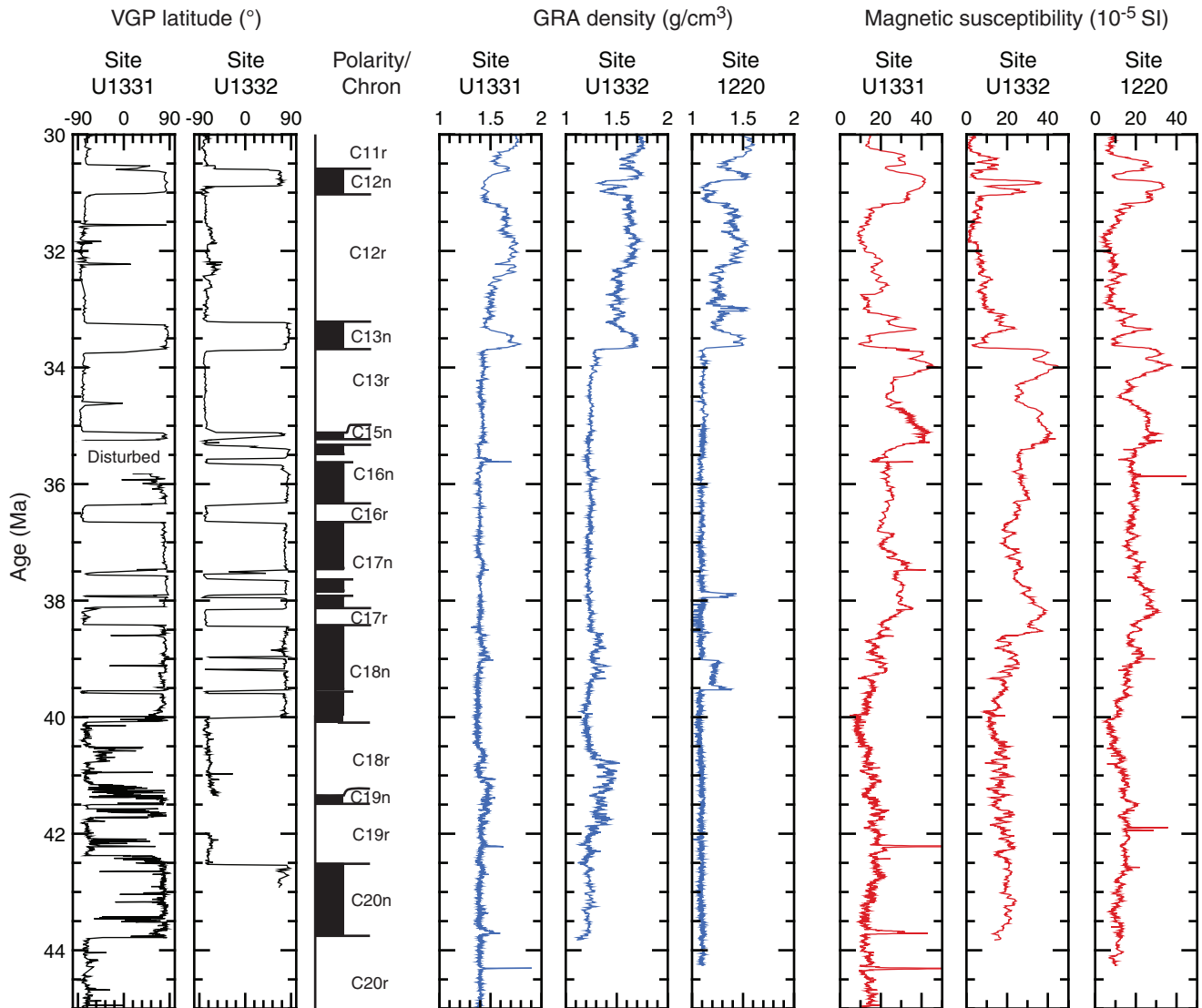
Figure F26. Coherence of sediment properties between widely separated drill sites from ODP Leg 199 and Expedition 320 in the equatorial Pacific is very high, allowing correlation of sediment properties over hundreds of kilometers. ODP Site 1220 and Expedition 320 Sites U1331 and U1332 are compared from 45 to 30 Ma. VGP = virtual geomagnetic pole. GRA density = gamma ray attenuation density (estimated on board).
