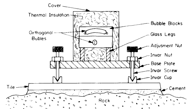
FIG. 3. A cut-away view of the tiltmeter used for volcano monitoring.
