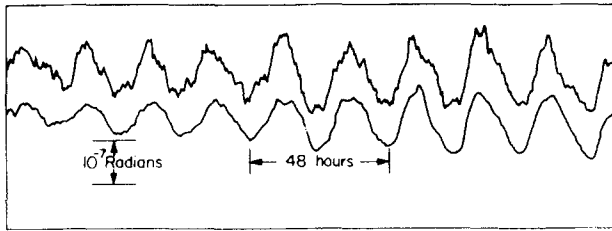
FIG. 4. Comparison of earth tide investigation records from the Fredericks (upper) and Rockwell (lower) bubble tilt sensors.
