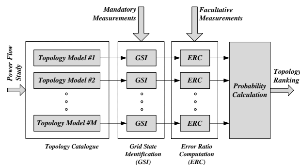
Fig. 1: Concept of the topology-recognition algorithm
