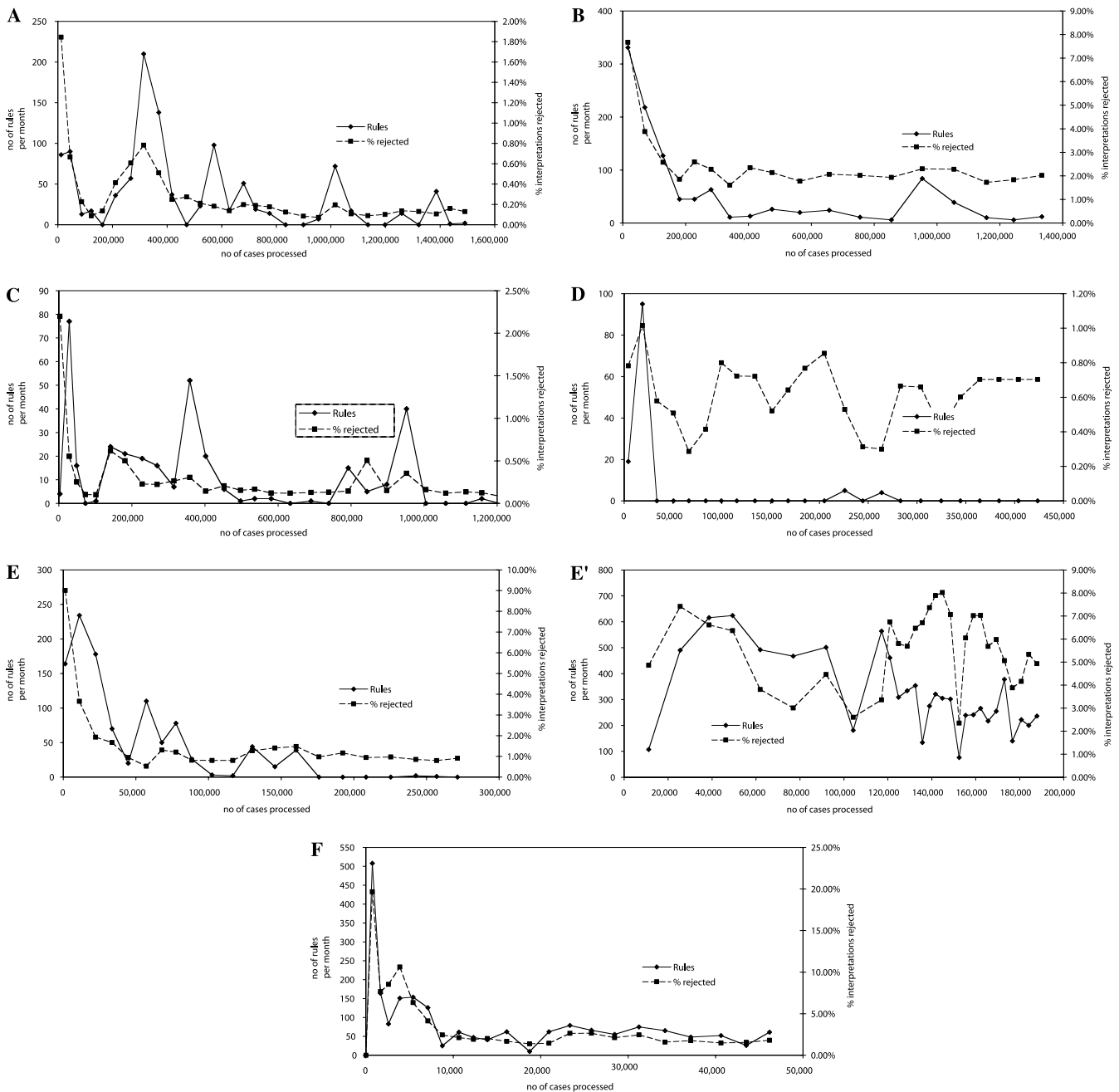
Fig. 6. A selection of knowledge bases, showing the number of rules added per month and the percentage of reports rejected, i.e., where the comments are edited before reports go out, against the number of cases processed.
