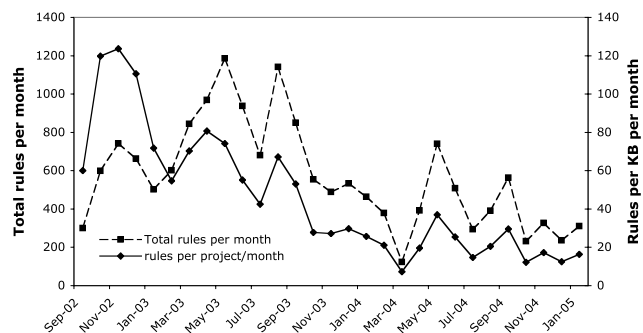
Fig. 4. The rate at which rules are added both across the whole laboratory and per KB.
