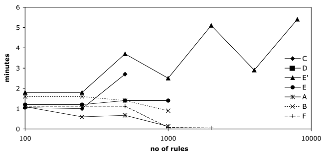
Fig. 5. The average time taken to add a rule at different KB sizes for some sample KBS.
