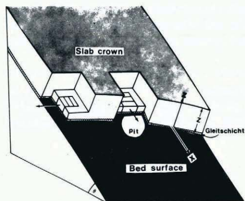
Fig. 2. Cross-slope and down-slope orientation of shear frame at crown of snow slab.
