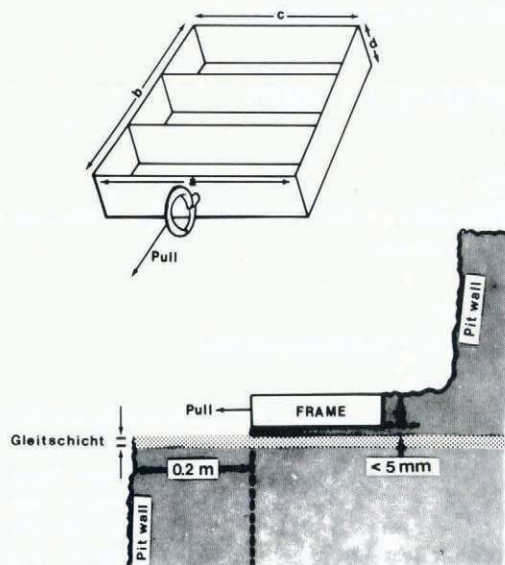
Fig. 1. The shear frame and its alignment on the Gleitschicht.
