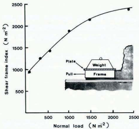
Fig. 3. Typical data which show the increase in the shear frame index with normal load. Each data point is based on the average of five measurements on a layer of partially metamorphosed crystals \rho = 200 \text{ kg m}^{-3} .
