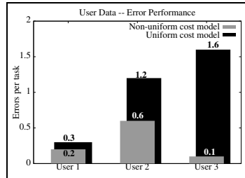
Figure 6: Empirical comparison between uniform and non-uniform cost models. Results are an average over 10 tasks. Depicted are 3 example users, with varying levels of speech recognition accuracy. Users 2 & 3 had the lowest recognition accuracy, and consequently more errors when using the uniform cost model.
