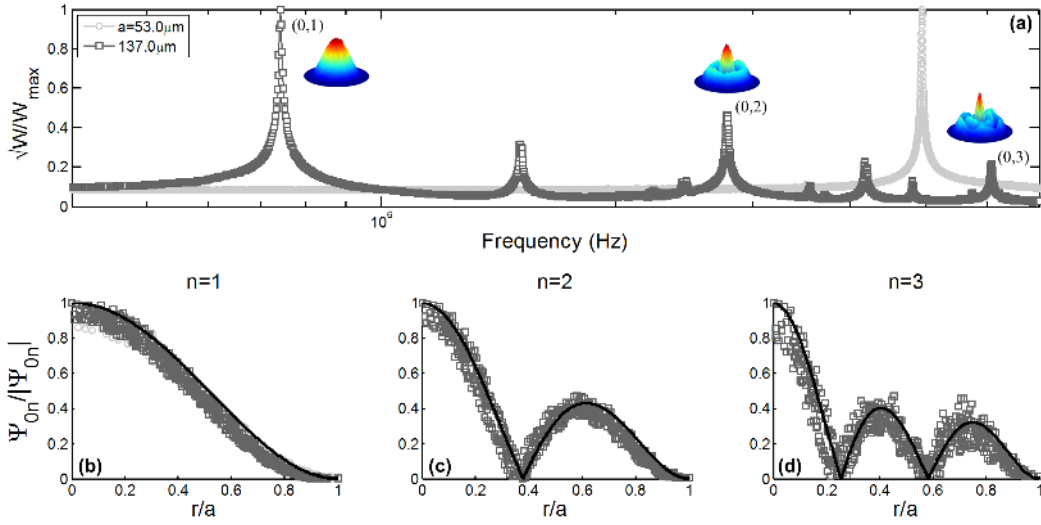
Fig. 11. LDV frequency sweep measurement normalized to deflection at fundamental resonant mode (a), insets show 3D views of raw profile data (axes not to scale) for a = 137.0\mu m device at each axisymmetric mode. Normalized profile slices as a function of dimensionless radius compared to shape profile in Equation 4 for n = 1, 2, 3 axisymmetric vibration modes shown in (b)-(d), respectively.
