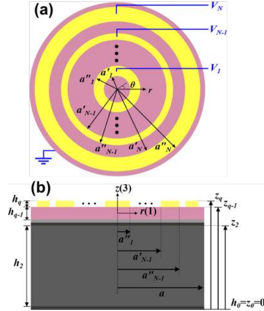
Fig. 2. Top (a) and cross-section (b) schematic of N electrode pMUT consisting of q material layers. Stack thickness z_i determined by thickness of i^{\text{th}} layer h_i and preceding layers according to Appendix A .
