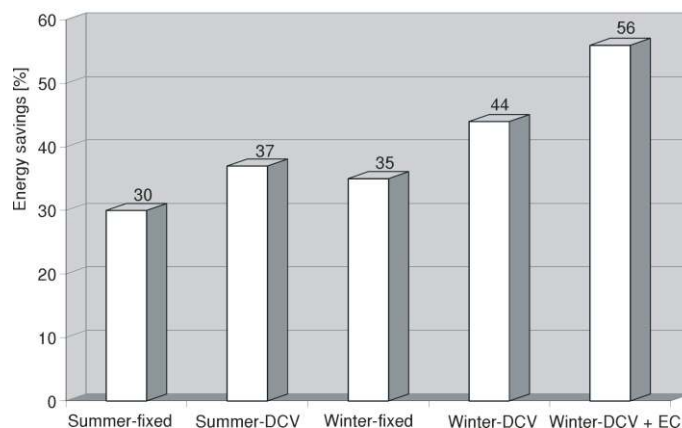
Figure 16. Energy-saving potential of VRV-VAV A/C system
