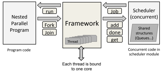
Figure 3: Interface for the program and scheduling modules.
