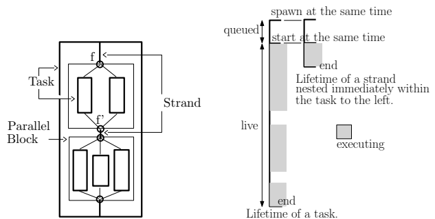
Figure 2: (left) Decomposing the computation: tasks, strands and parallel blocks. f, f' are corresponding fork and join points. (right) Timeline of a task and its first strand, showing the difference between being live and execution.
