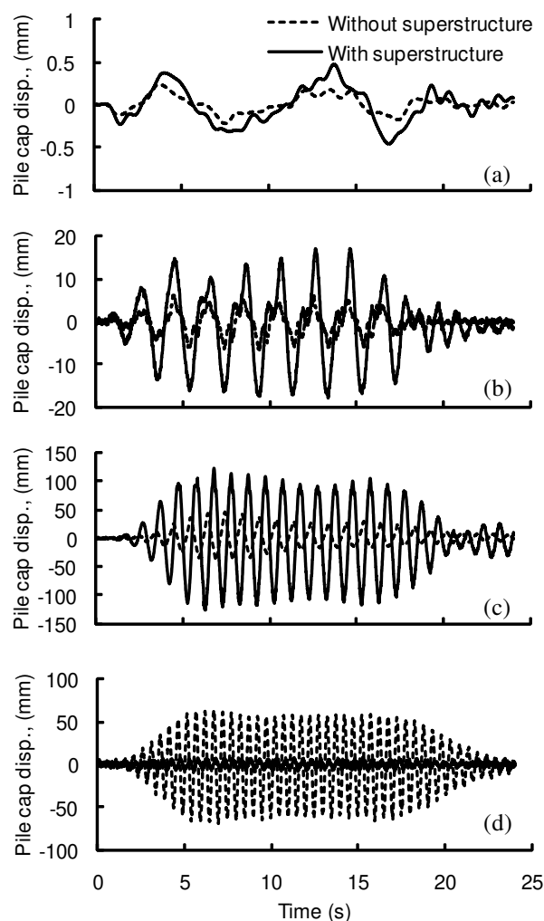
Fig.3 Time histories of pile cap displacement; 0.1 Hz (a), 0.5 Hz (b), 1.0 Hz (c) and 2.0 Hz (d)
